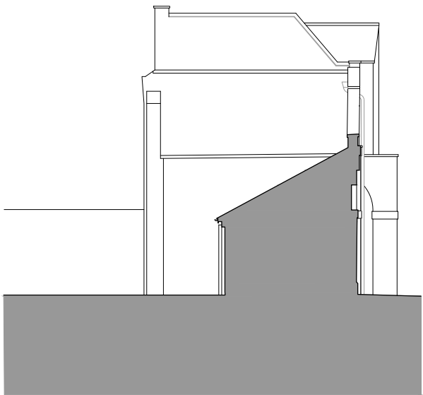
B WEST ELEVATION (EAST STABLES BLOCK) 511 AS EXISTING
