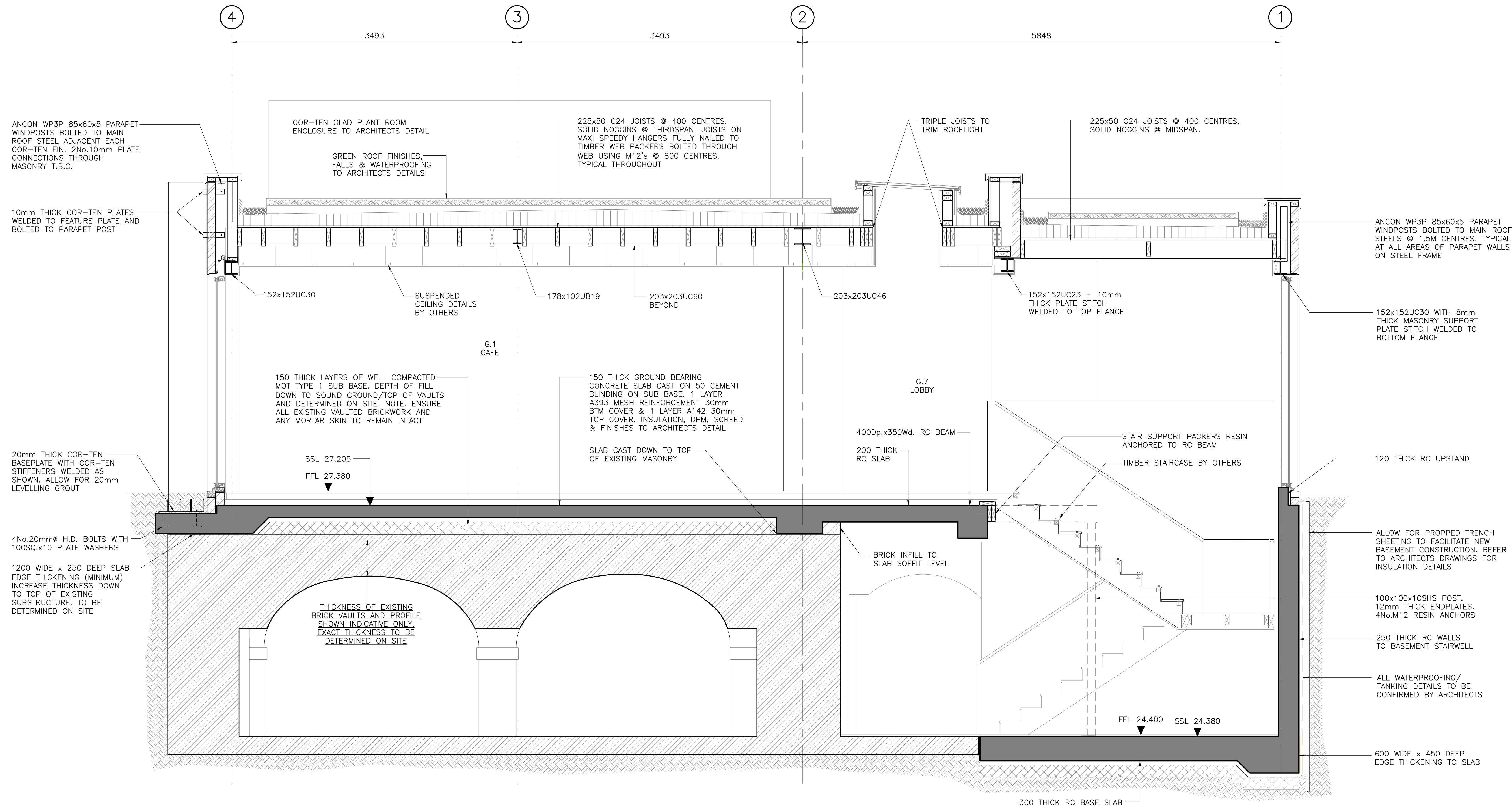
SECTION B – B
