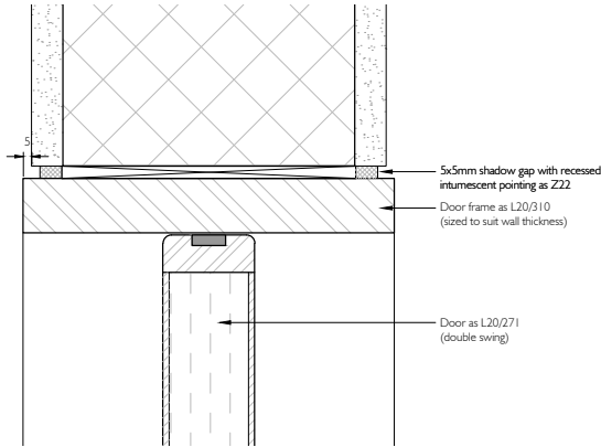
3 DOOR TYPE 5 - HEAD DETAIL
