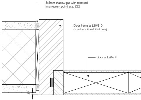
4 DOOR TYPES 6, 7 & 9 - JAMB DETAIL
