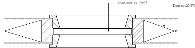
5 DOOR TYPE 6 - VISION PANEL DETAIL
