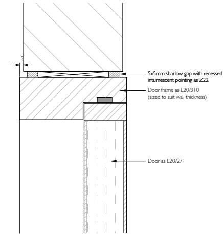
10 DOOR TYPE 11 - HEAD DETAIL
