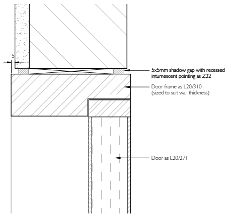
8 DOOR TYPE 8 & 10 - HEAD DETAIL
