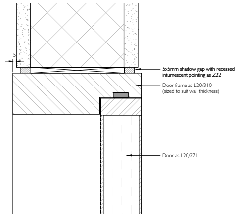
6 DOOR TYPES 6, 7 & 9 - HEAD DETAIL
