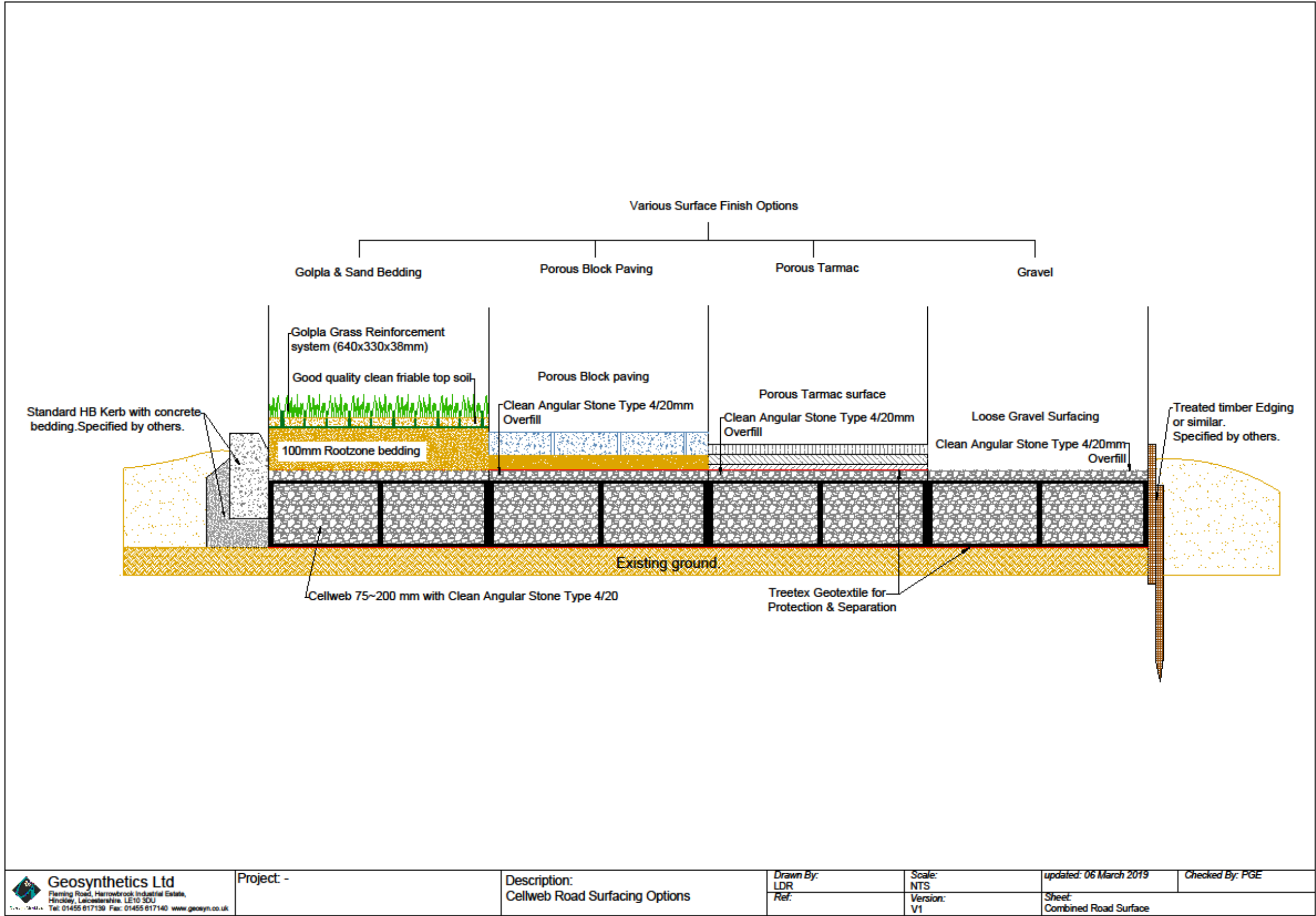
Figure 5- Example of potential support within RPAs with various upper surface finishes (if needed)
