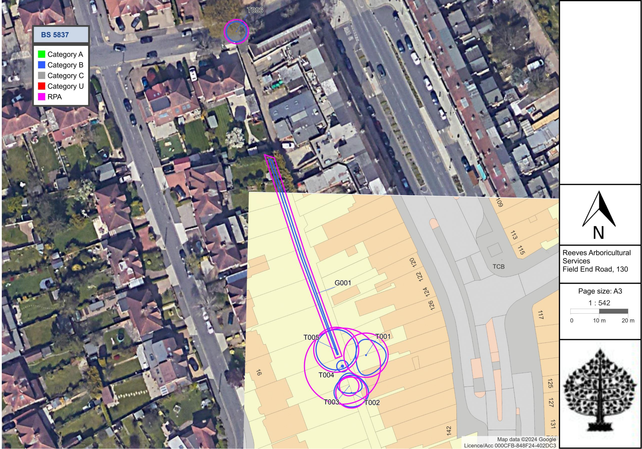
Tree constraints plan- ASIAMS202-M02
