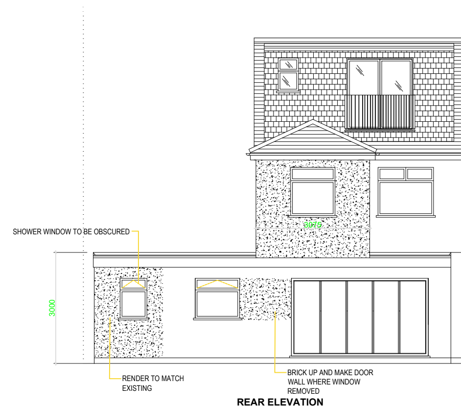
REAR ELEVATION
