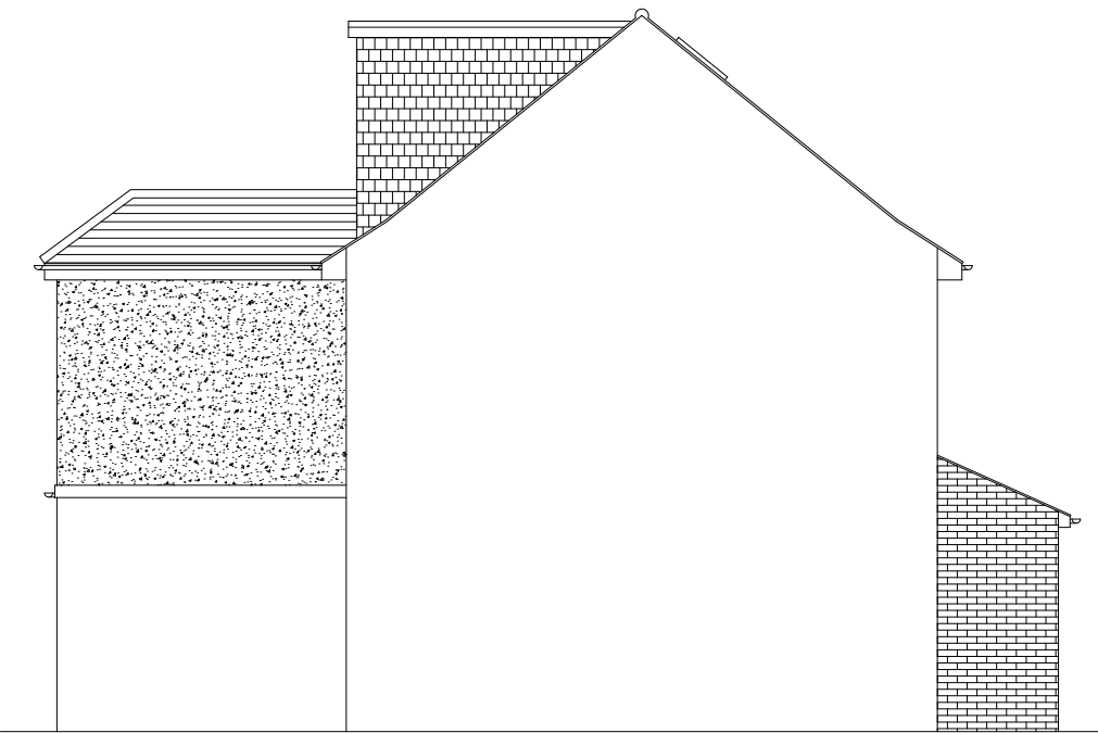
SIDE ELEVATIONS
