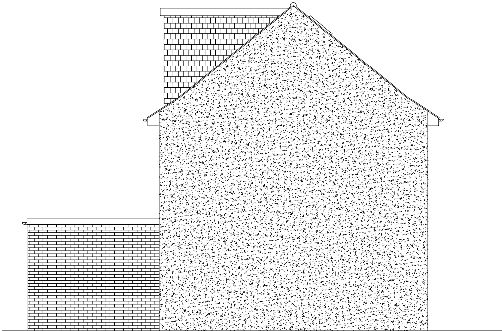
SIDE ELEVATIONS
