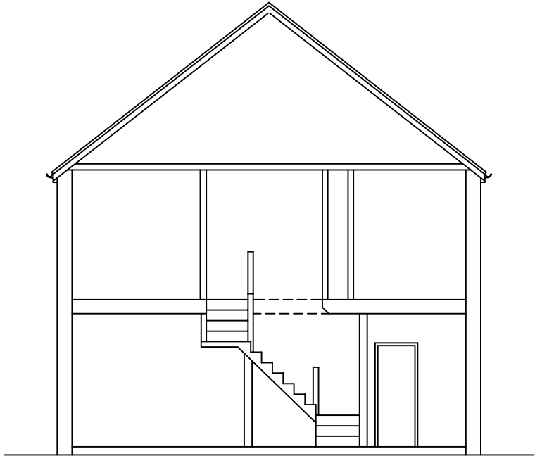
EXISTING STAIR CROSS-SECTION
