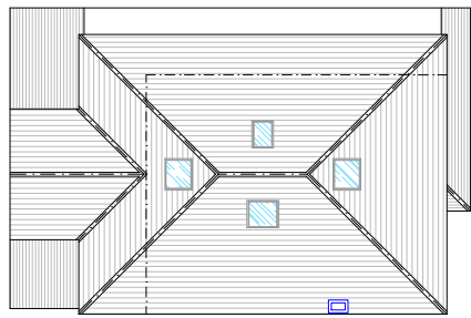
PROPOSED ROOF PLAN SCALE 1/100
