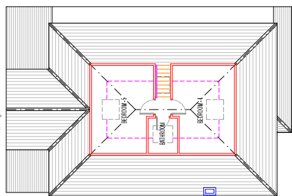
PROPOSED LOFT FLOOR PLAN SCALE 1/100
