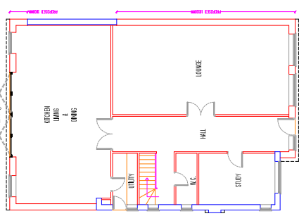
PROPOSED GROUND FLOOR PLAN SCALE 1/100
