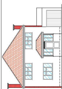
EXISTING FRONT ELEVATION SCALE 1/100
