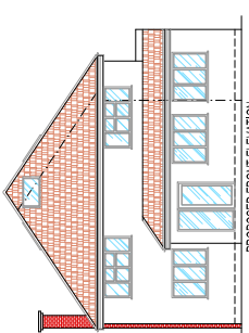
PROPOSED FRONT ELEVATION SCALE 1/100
