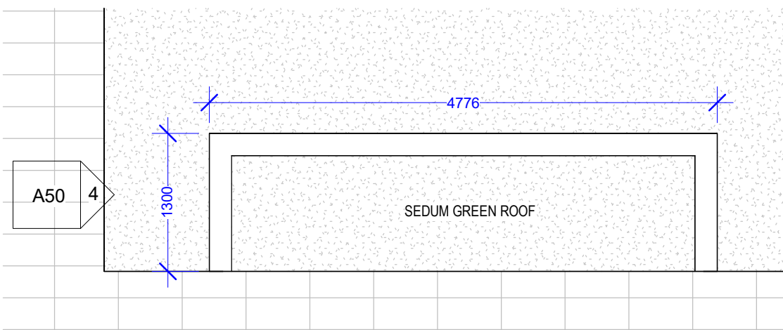
02 PROPOSED BIN / BIKE ROOF PLAN 1:50 @ A3
