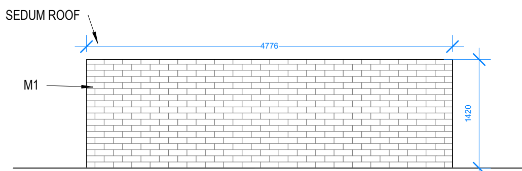
05 PROPOSED BIN / BIKE REAR ELEVATION 1:50 @ A3
