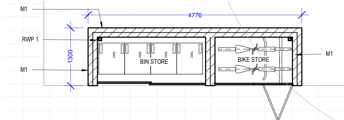
01 PROPOSED BIN / BIKE FLOOR PLAN 1:50 @ A3
