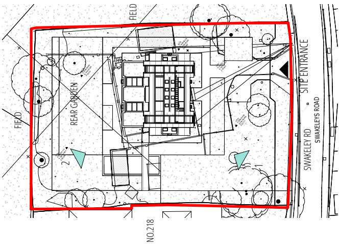
03 KEY PLAN 1:1000 @ A3
