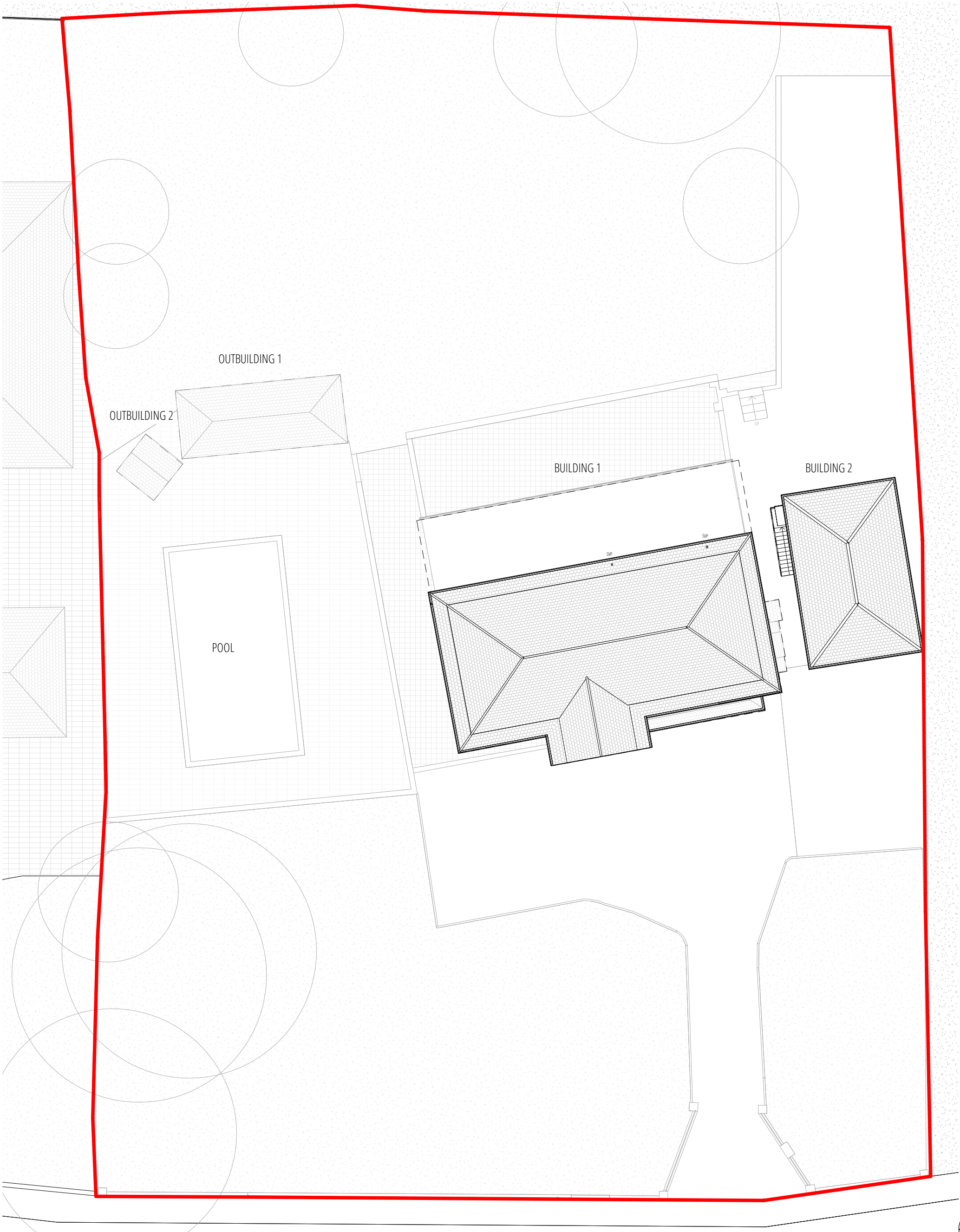
01 EXISTING ROOF PLAN 1:200 @ A3
