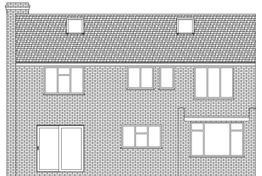
PROPOSED REAR ELEVATION REMAIN AS EXISTING
