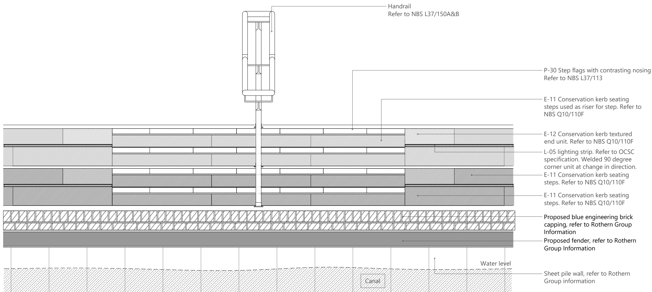
H7232-BOS-F3-00-DR-AL-90606 : D02 ELEVATION OF CANALSIDE STEPS SCALE: 1:10
