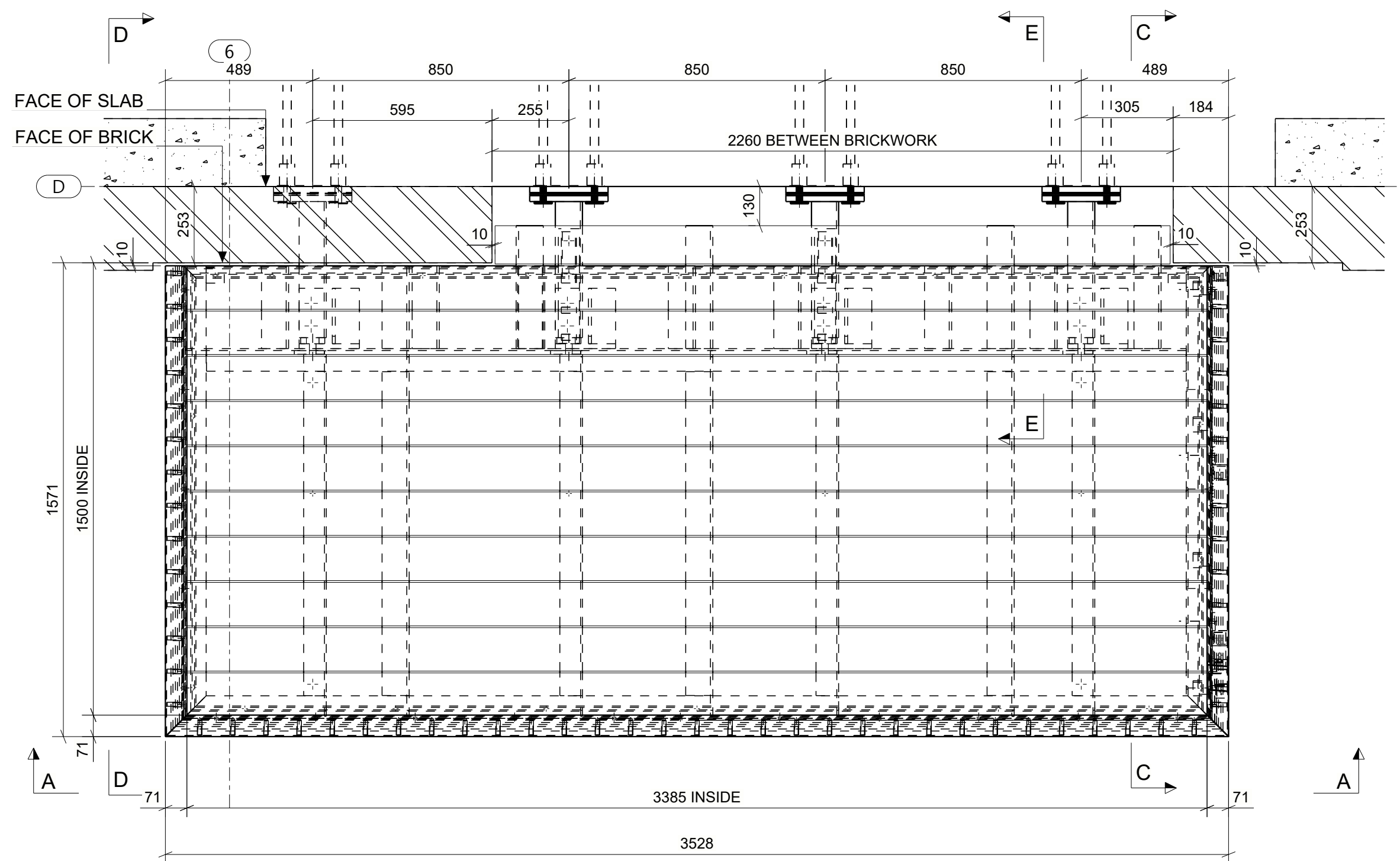
PLAN VIEW F3-AMT-04-01
