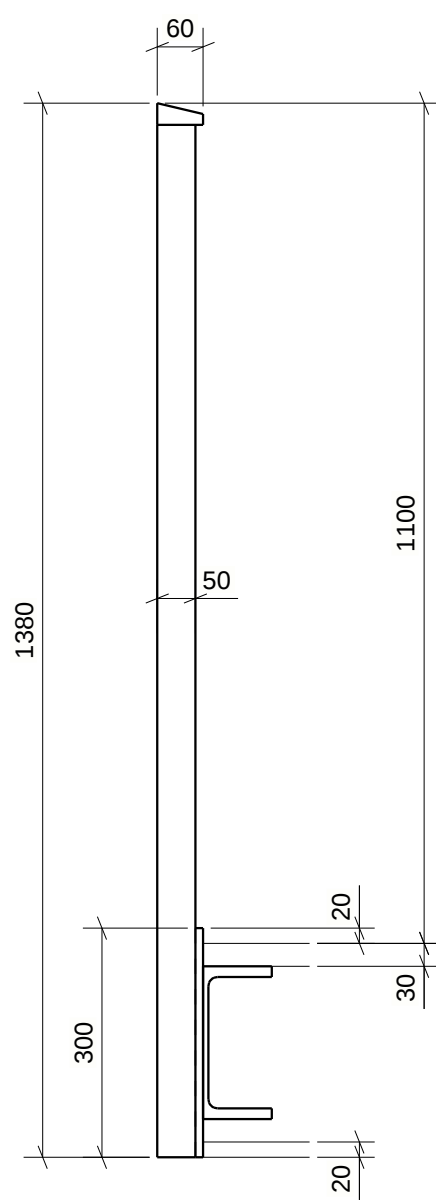
C - C SCALE 1:10
