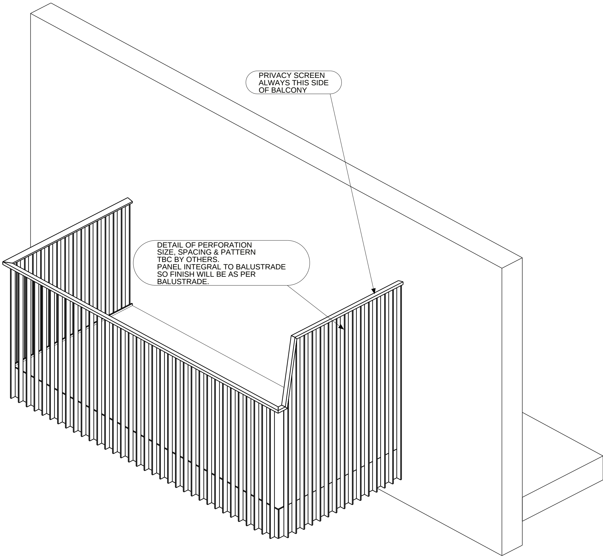
3D VIEW BALCONY F3 AMT-04
