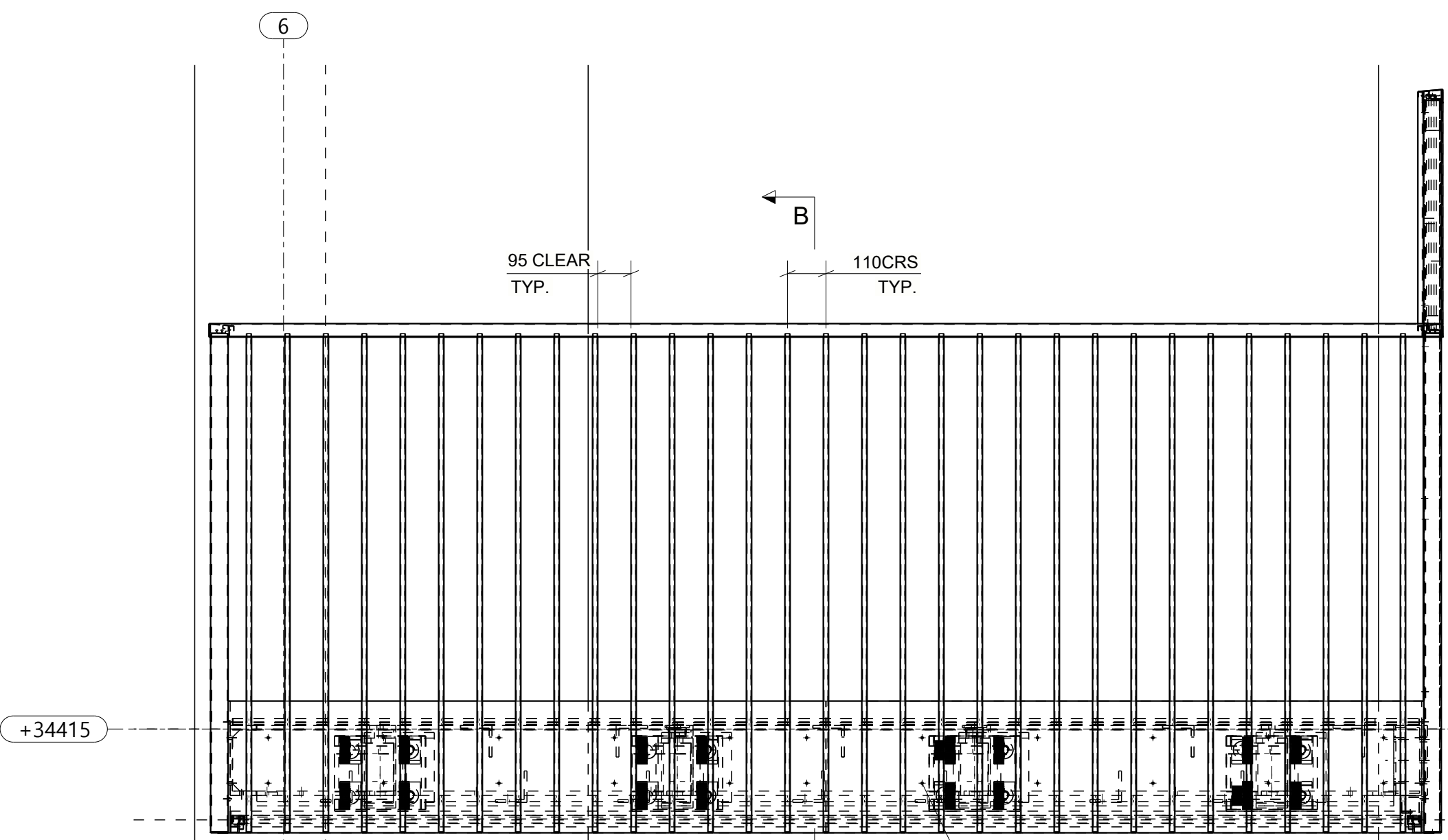
PLAN VIEW F3-AMT-04-01
