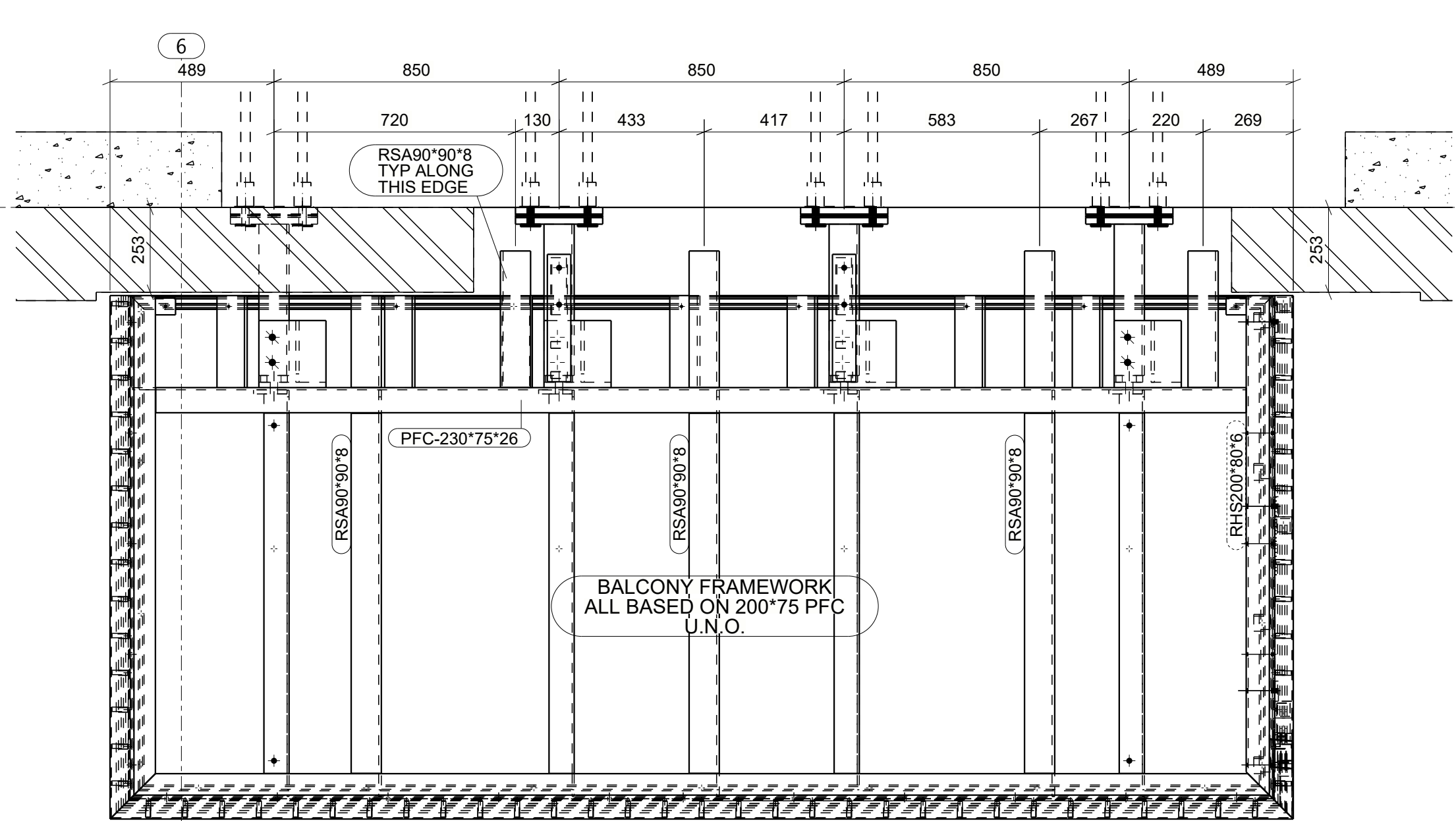
PLAN ON BALCONY (DECKING / SOFFIT OMITTED)
