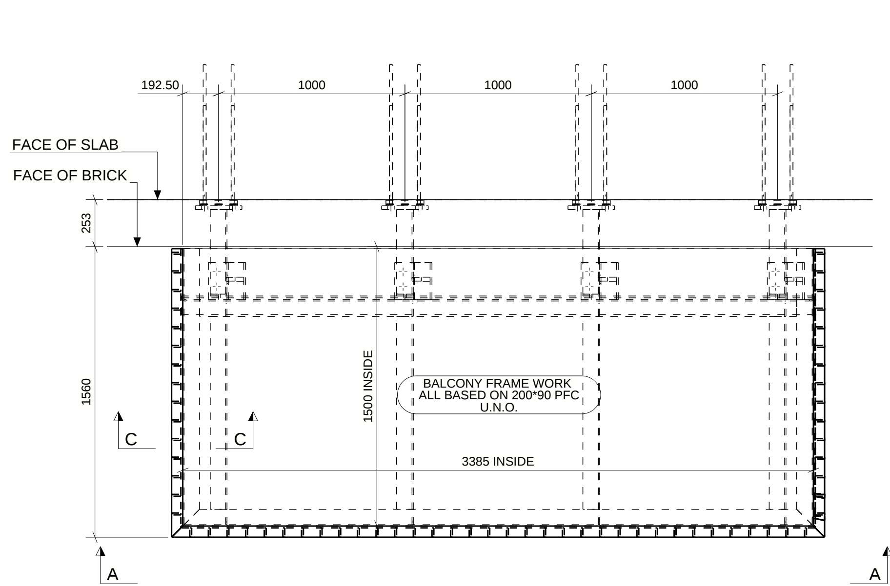
BALCONY TYPE F3 AMT-04 (253mm BRICKWORK)
