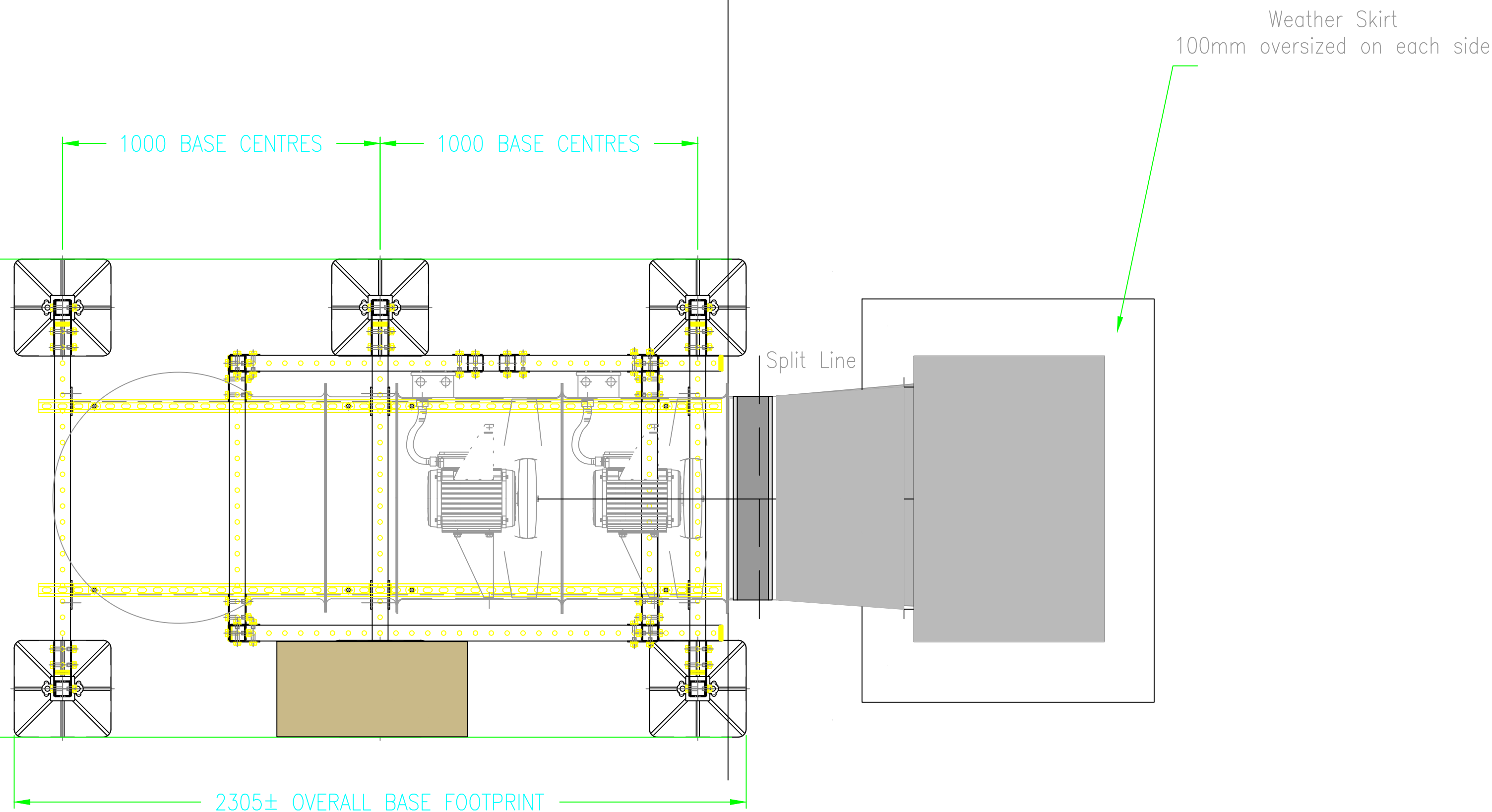
Plan View of Extract Shaft (External Dimensions)
