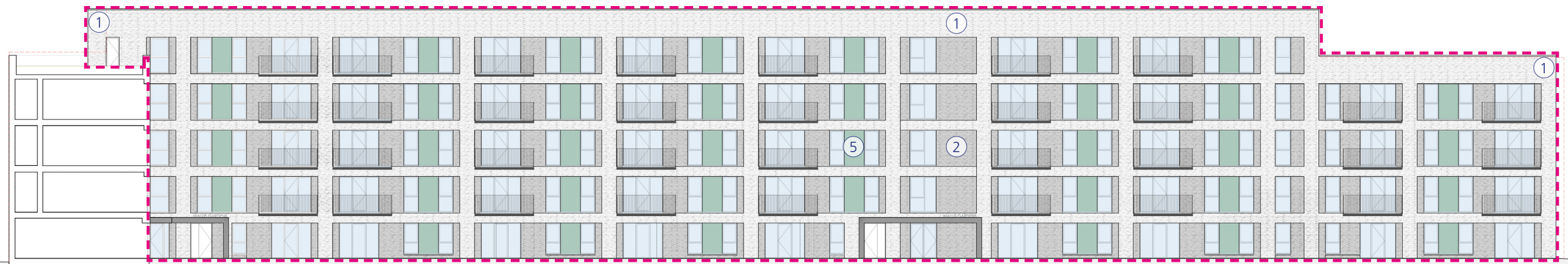
PROPOSED WEST ELEVATION (FACING WALLIS GARDENS)
