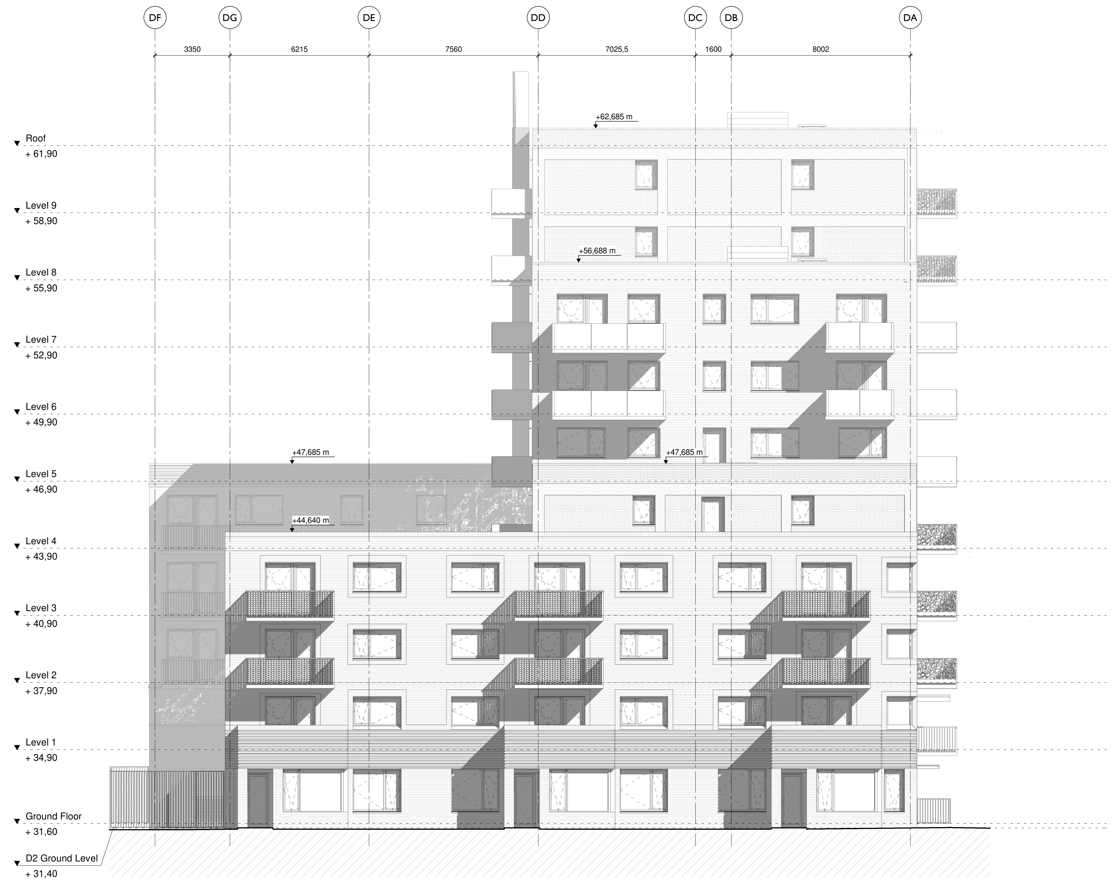
South Elevation 1 : 100
