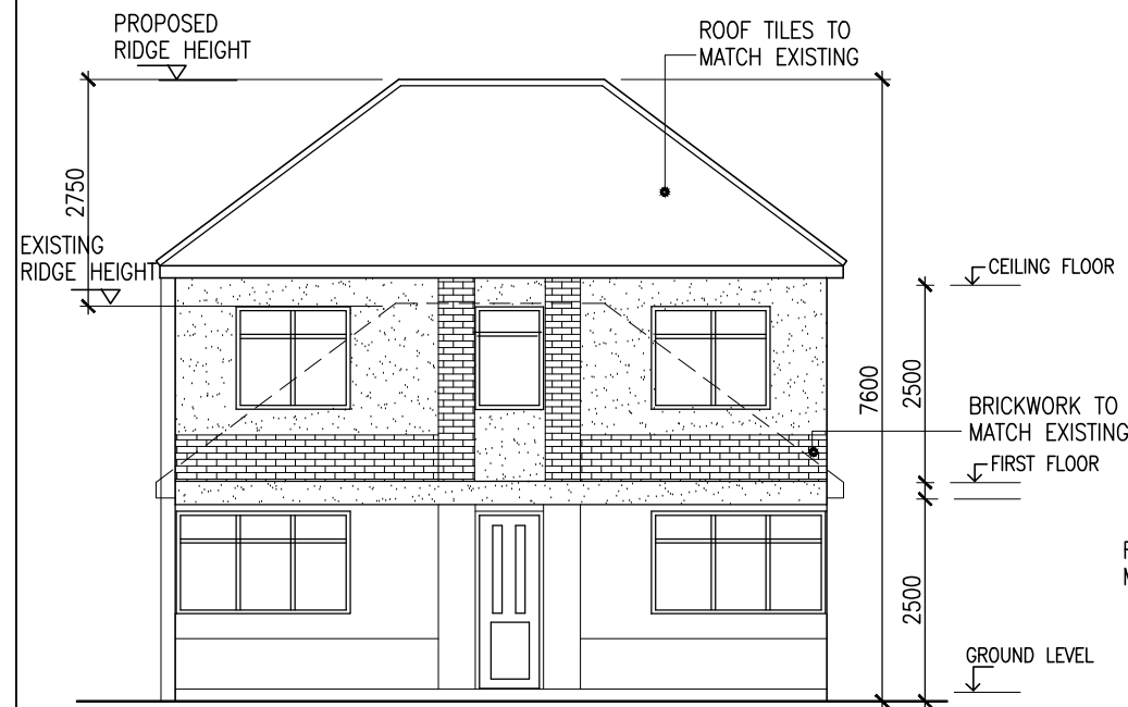
FRONT ELEVATION
