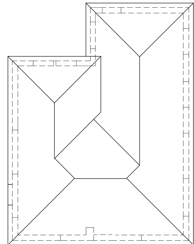
ROOF PLAN
