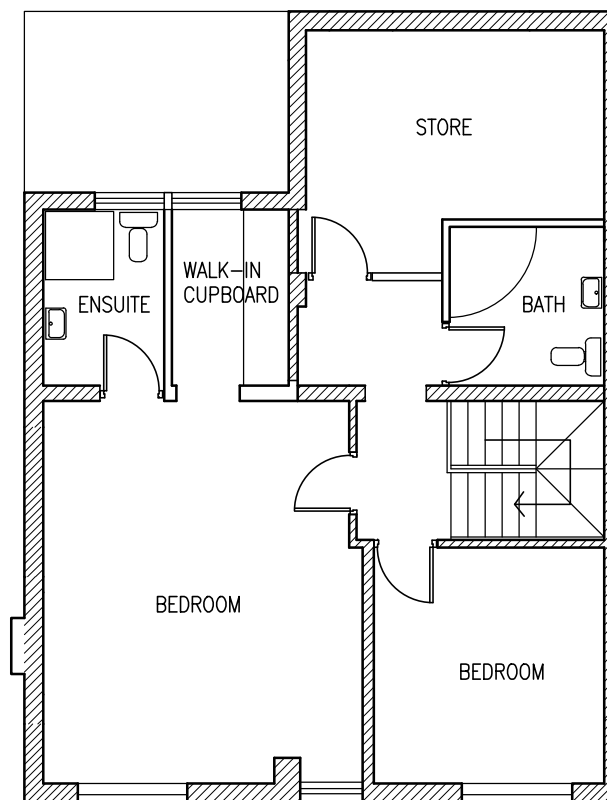
FIRST FLOOR PLAN – ADDITIONAL FLOOR
