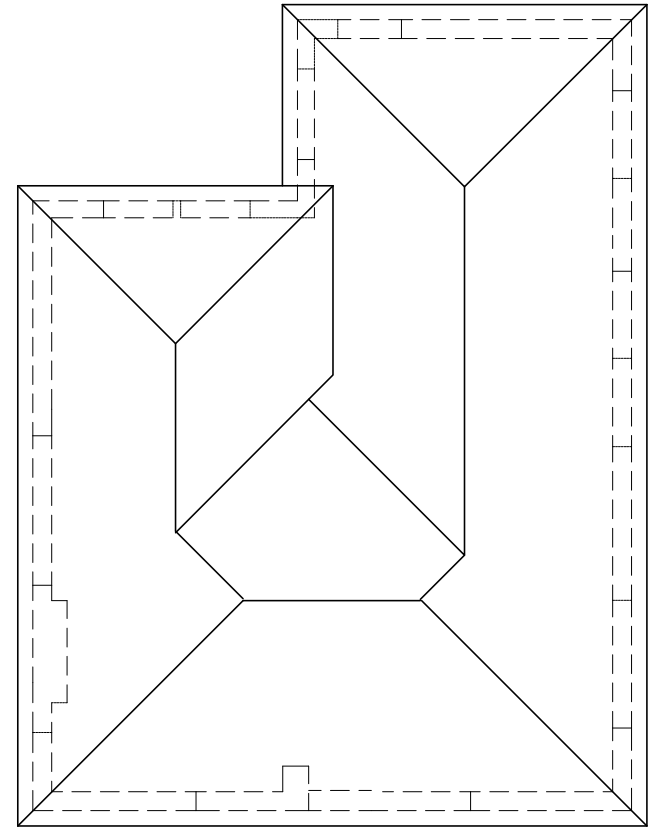
ROOF PLAN
