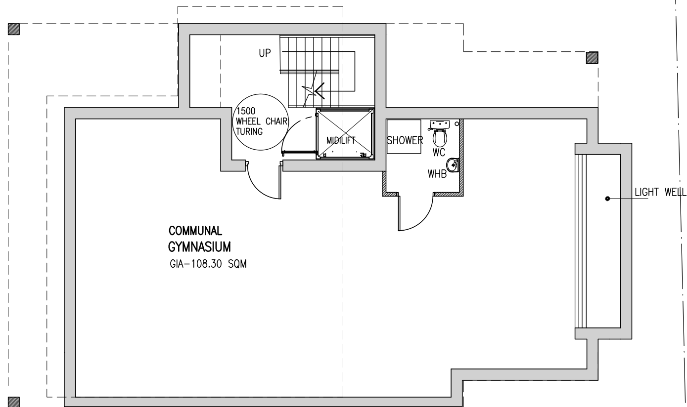
BASEMENT PLAN
