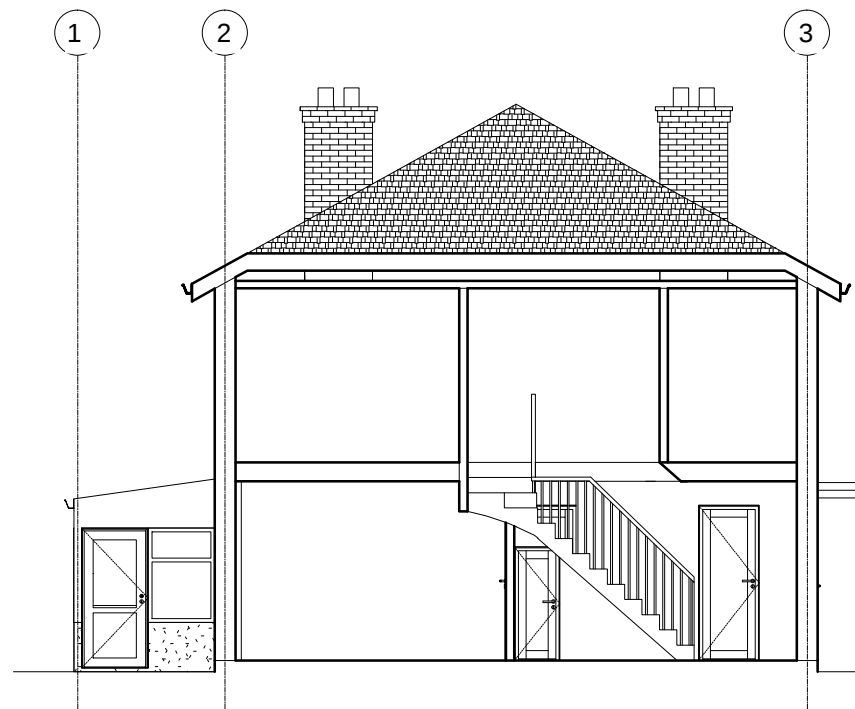
EXISTING SECTION
