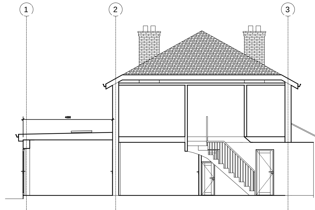
PROPOSED SECTION
