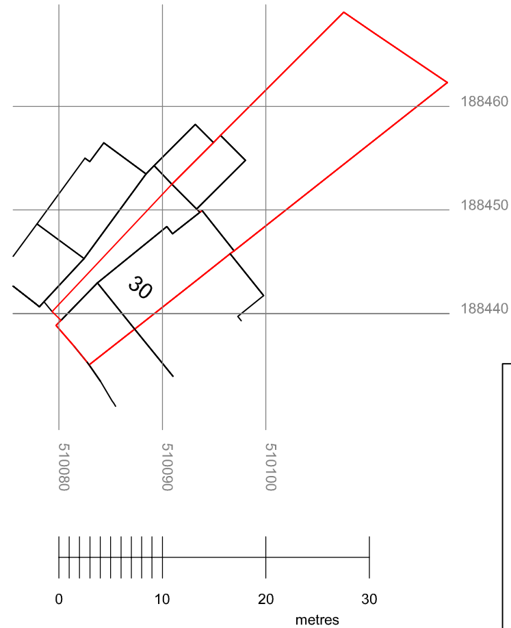
Block plan (1:500)
