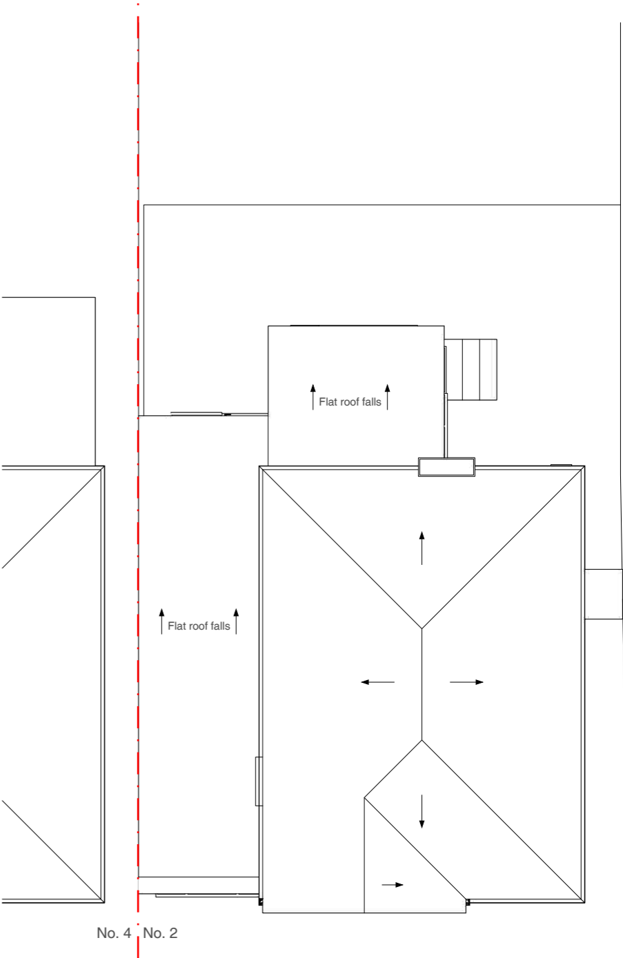
Roof Plan
