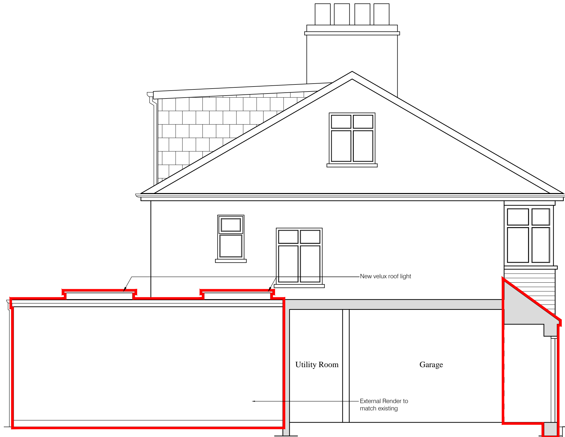
Proposed Side Elevation & Section
