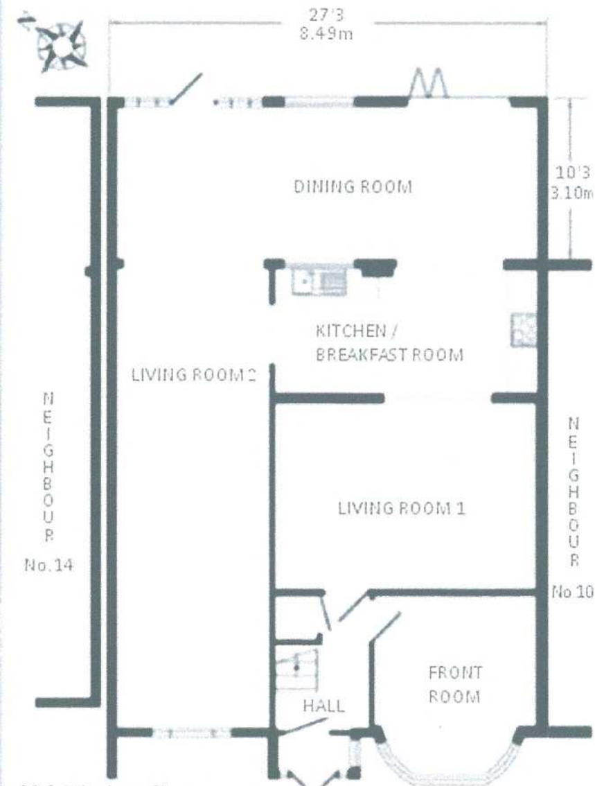
Fig 4 PROPOSED GROUND FLOOR
