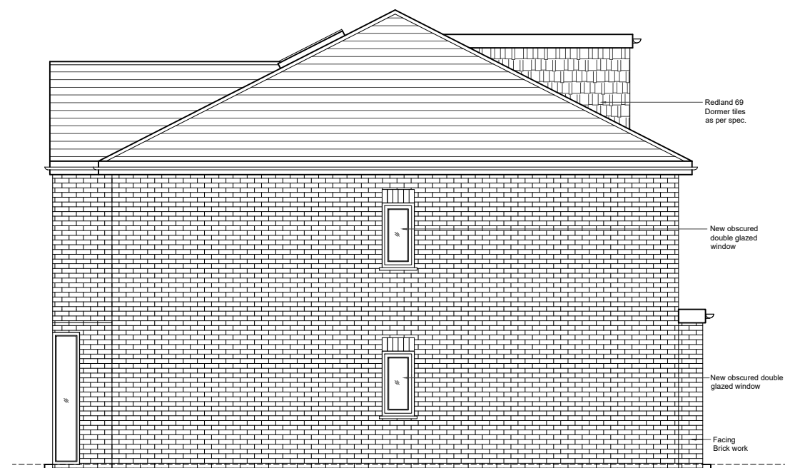
03 - RIGHT SIDE ELEVATION
