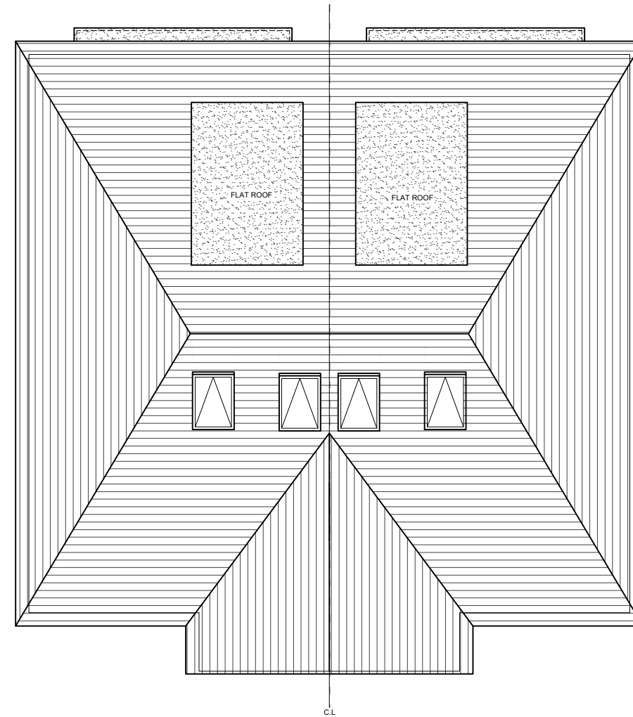
02 - ROOF PLAN
