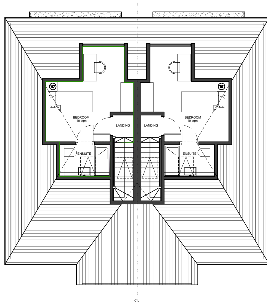
01 - LOFT FLOOR PLAN
