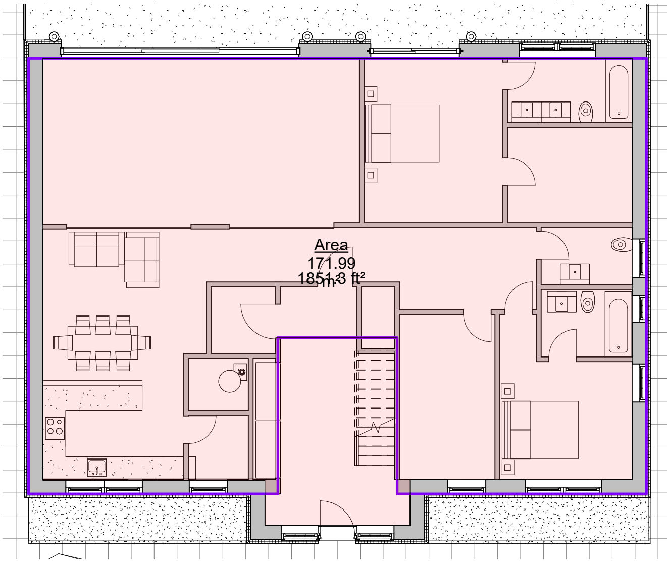
1 Ground Floor 1 : 100
