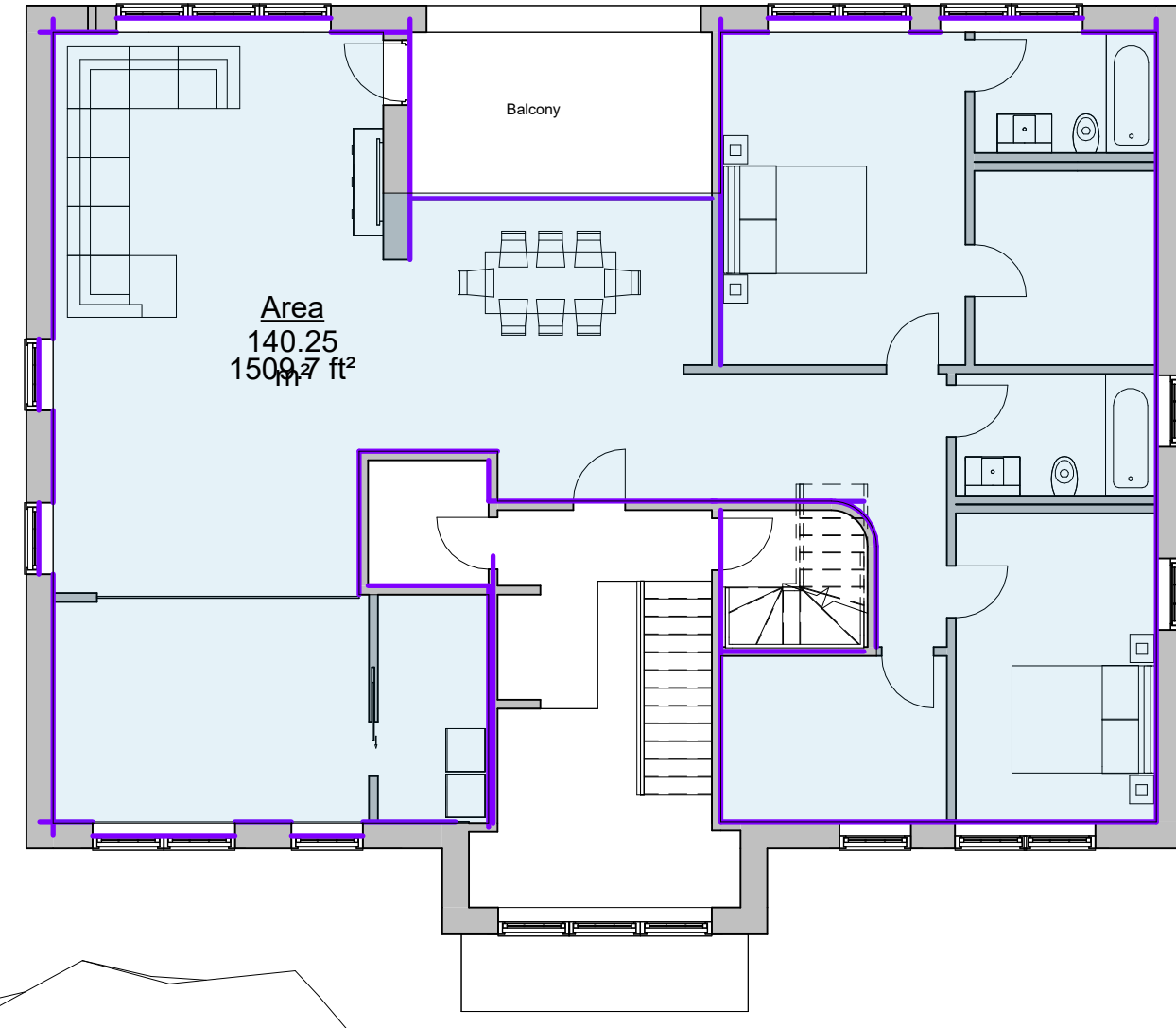
2 First Floor 1 : 100
