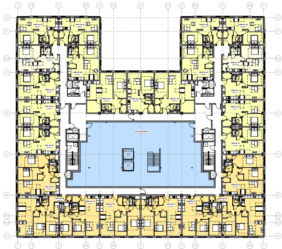
Figure 2.9 Second floor plan
