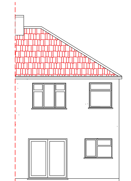
EXISTING REAR
