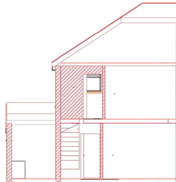
PROPOSED REAR SECTION
