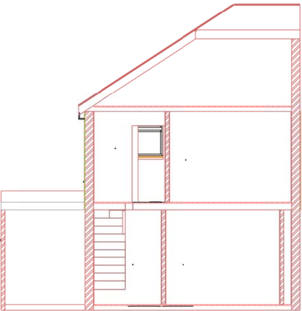
EXISTING REAR SECTION
