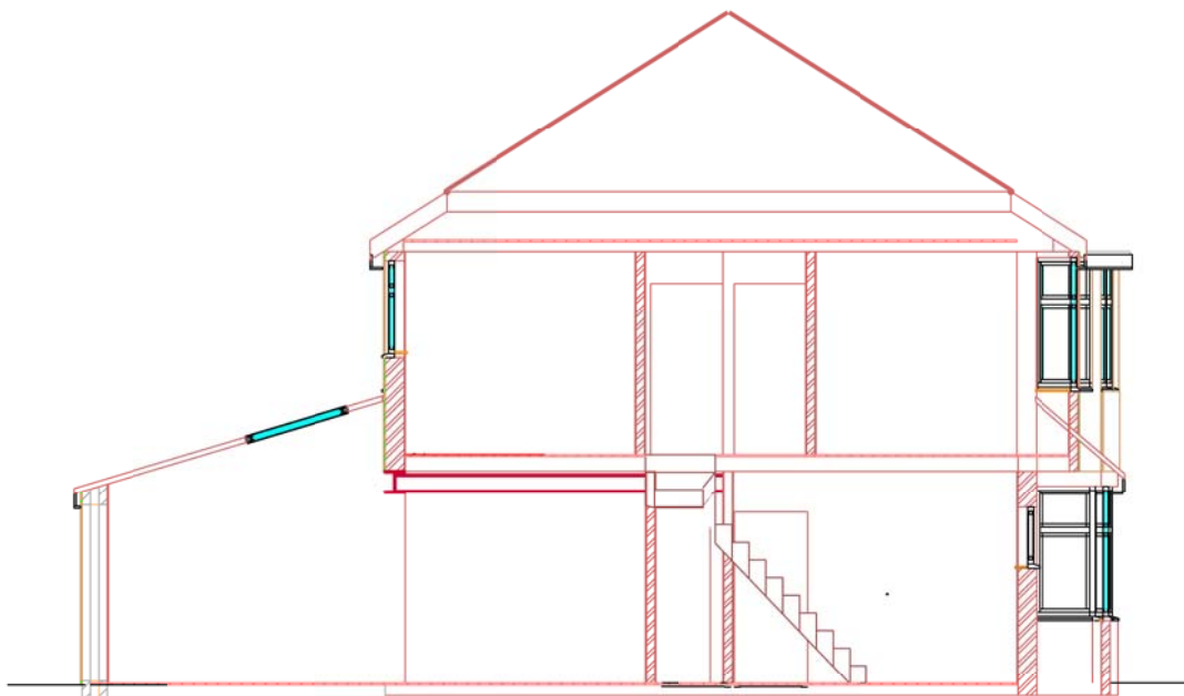
PROPOSED SIDE SECTION
