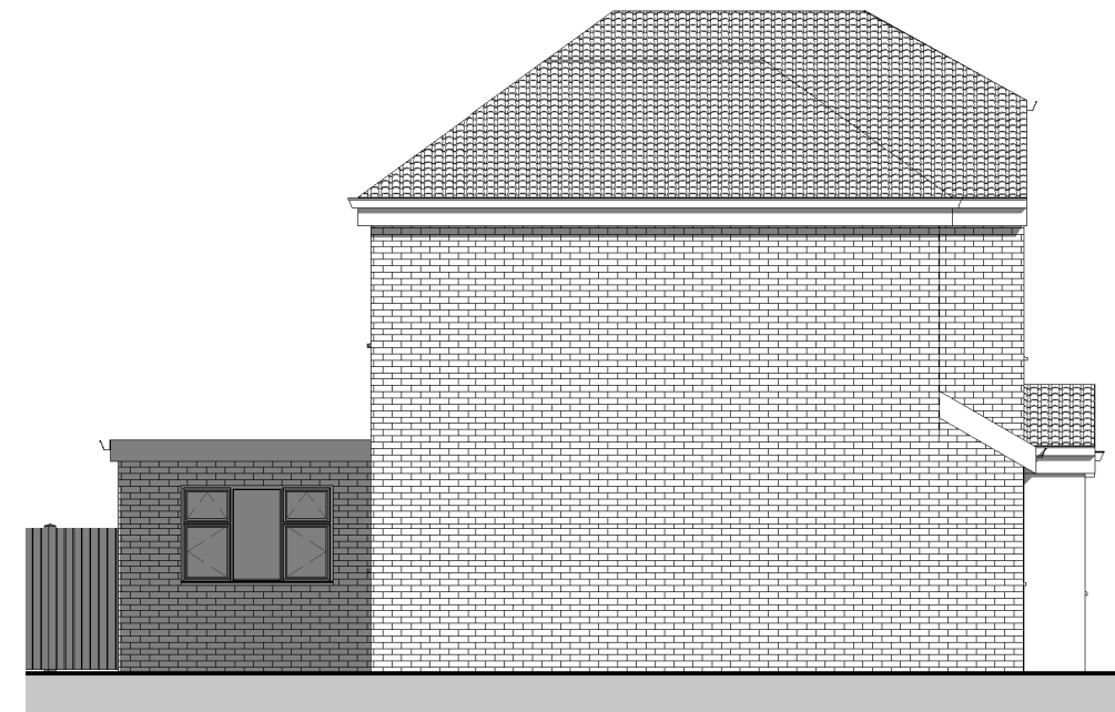
6 Proposed Side Elevation (West) 2112-A-600 1 : 100
