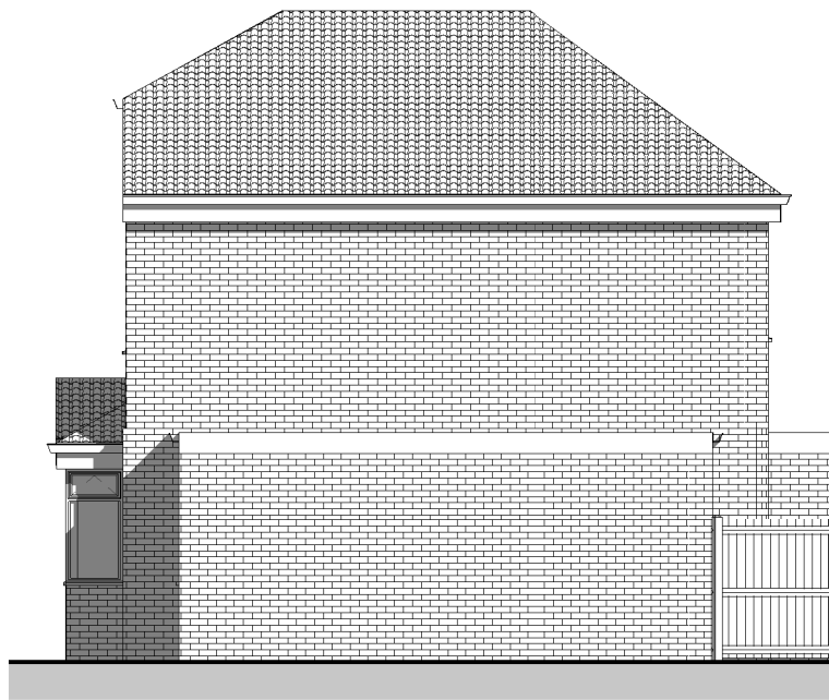
4 Proposed Side Elevation (East) 2112-A-600 1 : 100
