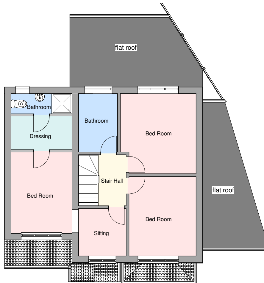
2 Proposed First Floor 2112-A-600 1 : 100
