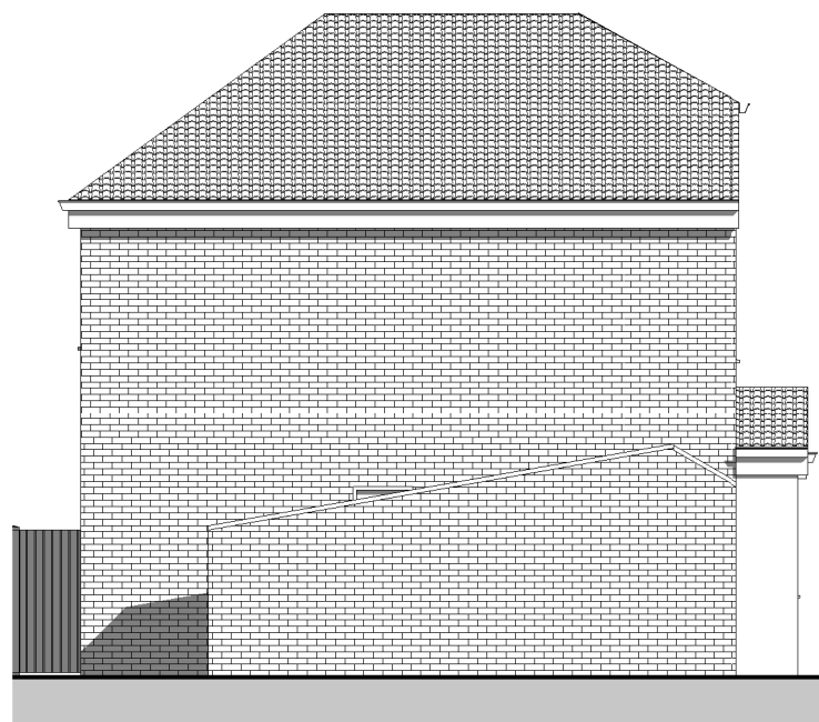
6 Existing Side Elevation (West) 2112-A-500 1 : 100
