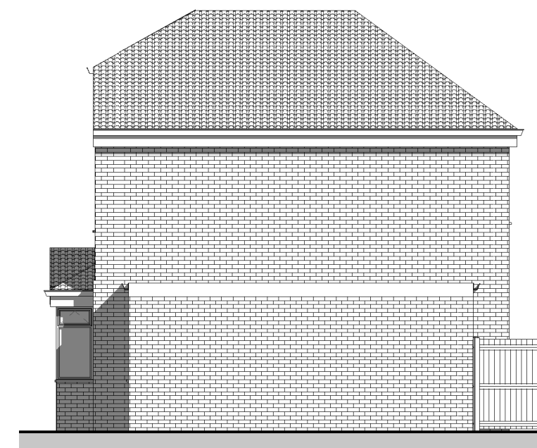
4 Existing Side Elevation (East) 2112-A-500 1 : 100
