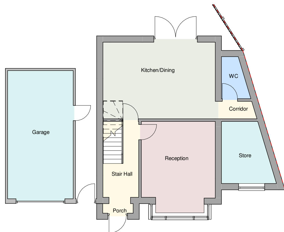
1 Existing Ground Floor 2112-A-500 1 : 100
