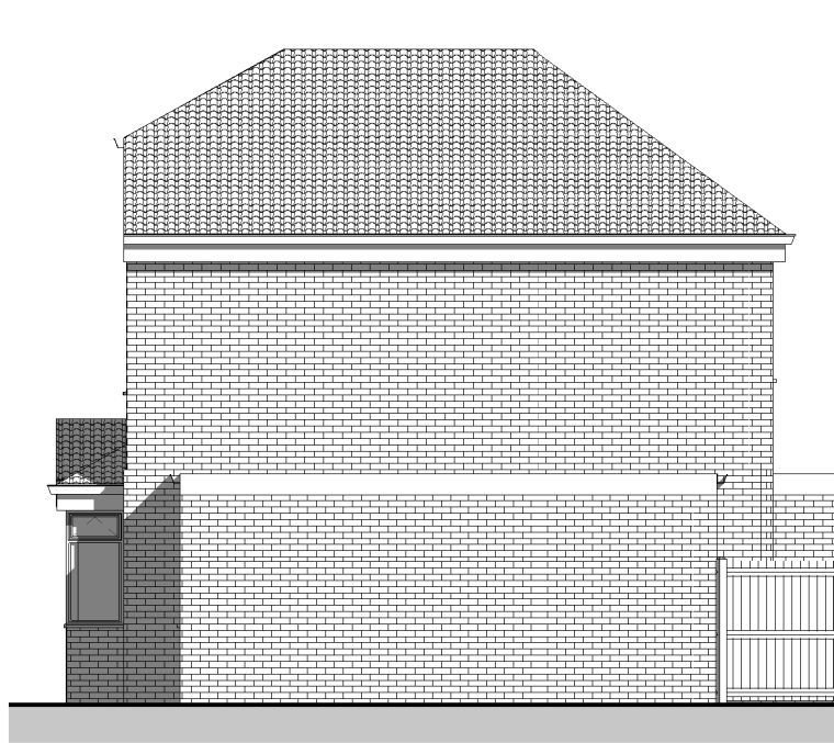
4 Proposed Side Elevation (East) 2112-A-600 1 : 100
