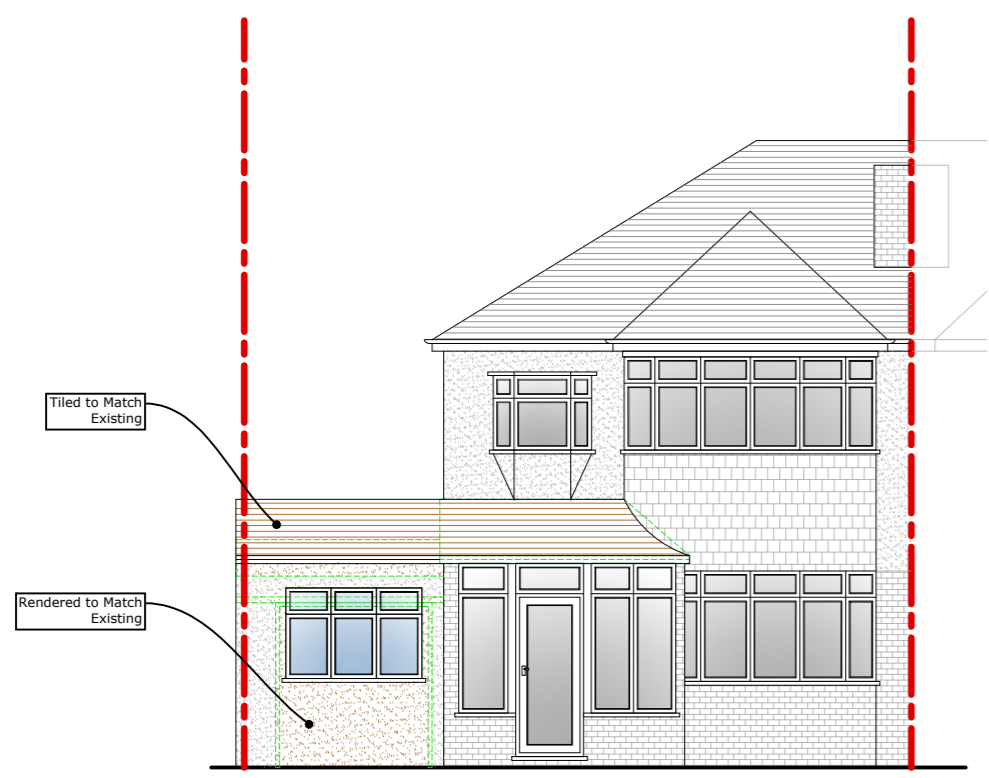
4 Proposed Front Elevation
