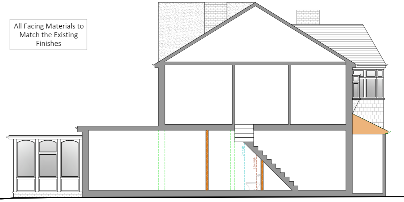
8 Proposed Side Section
