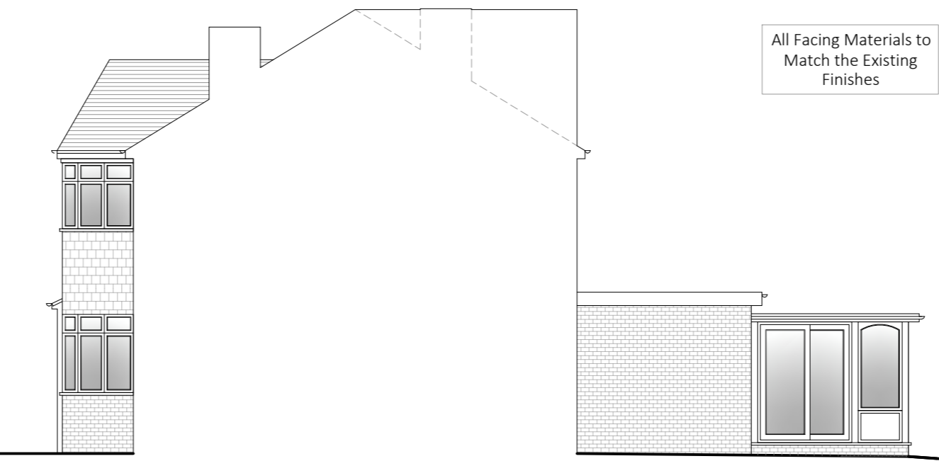
5 Proposed Side Elevation
