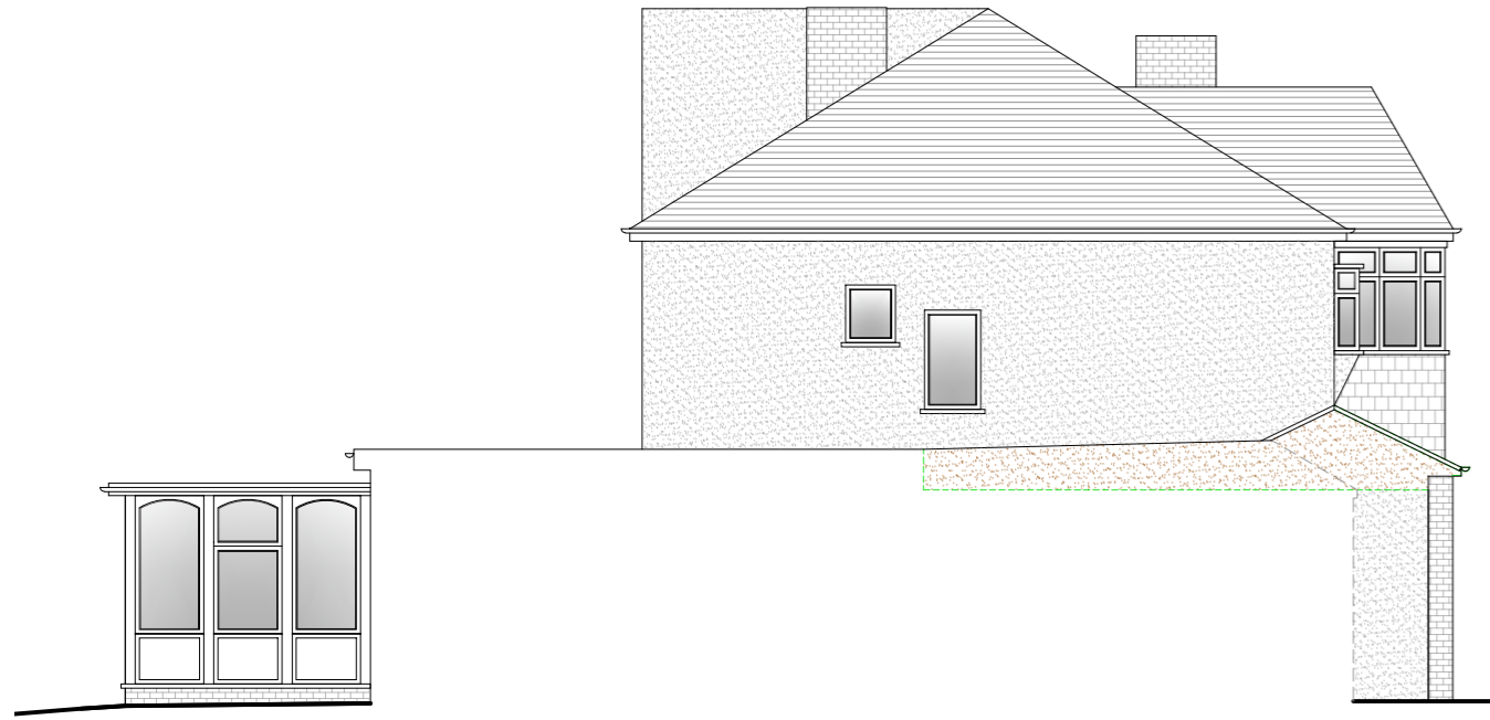
7 Proposed Side Elevation
