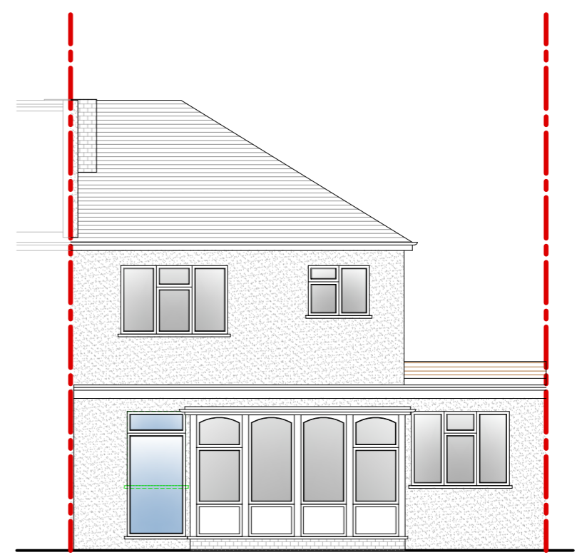
6 Proposed Rear Elevation
