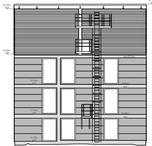
South Internal Elevation
