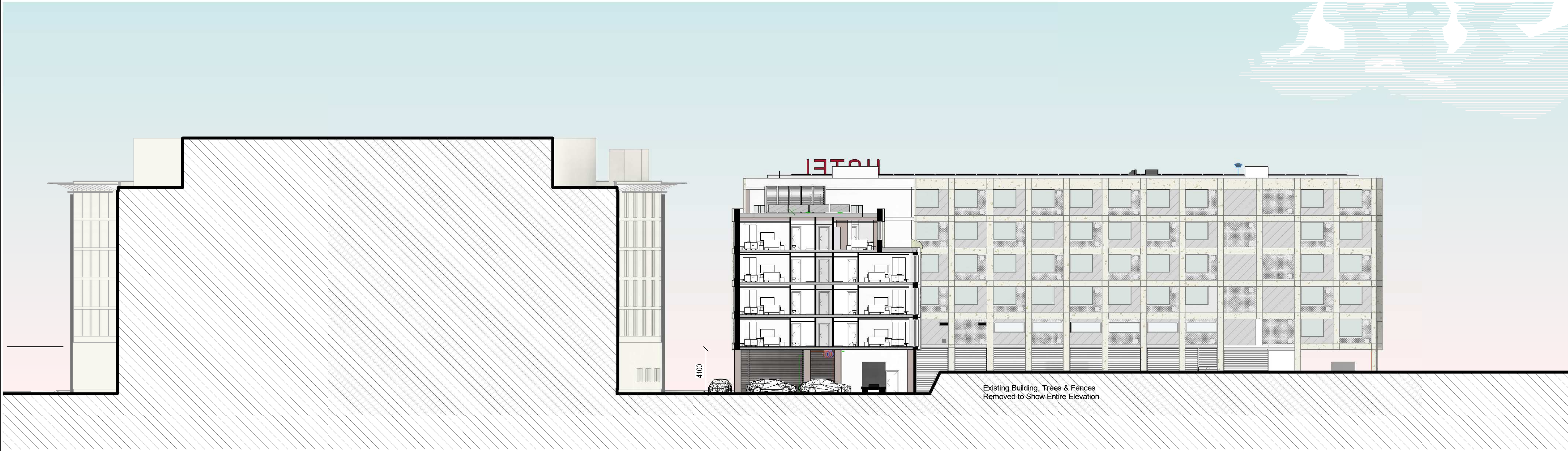
2 Section 3 1:200
