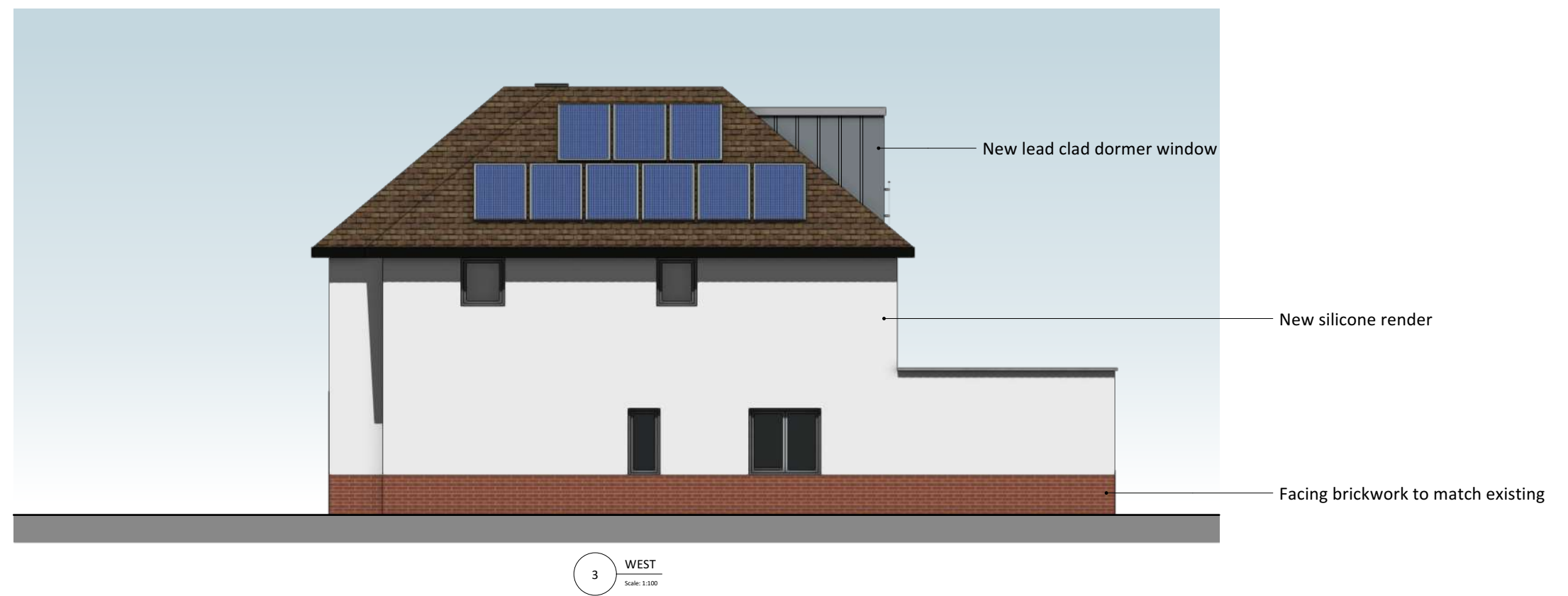
3 WEST Scale 1:100
