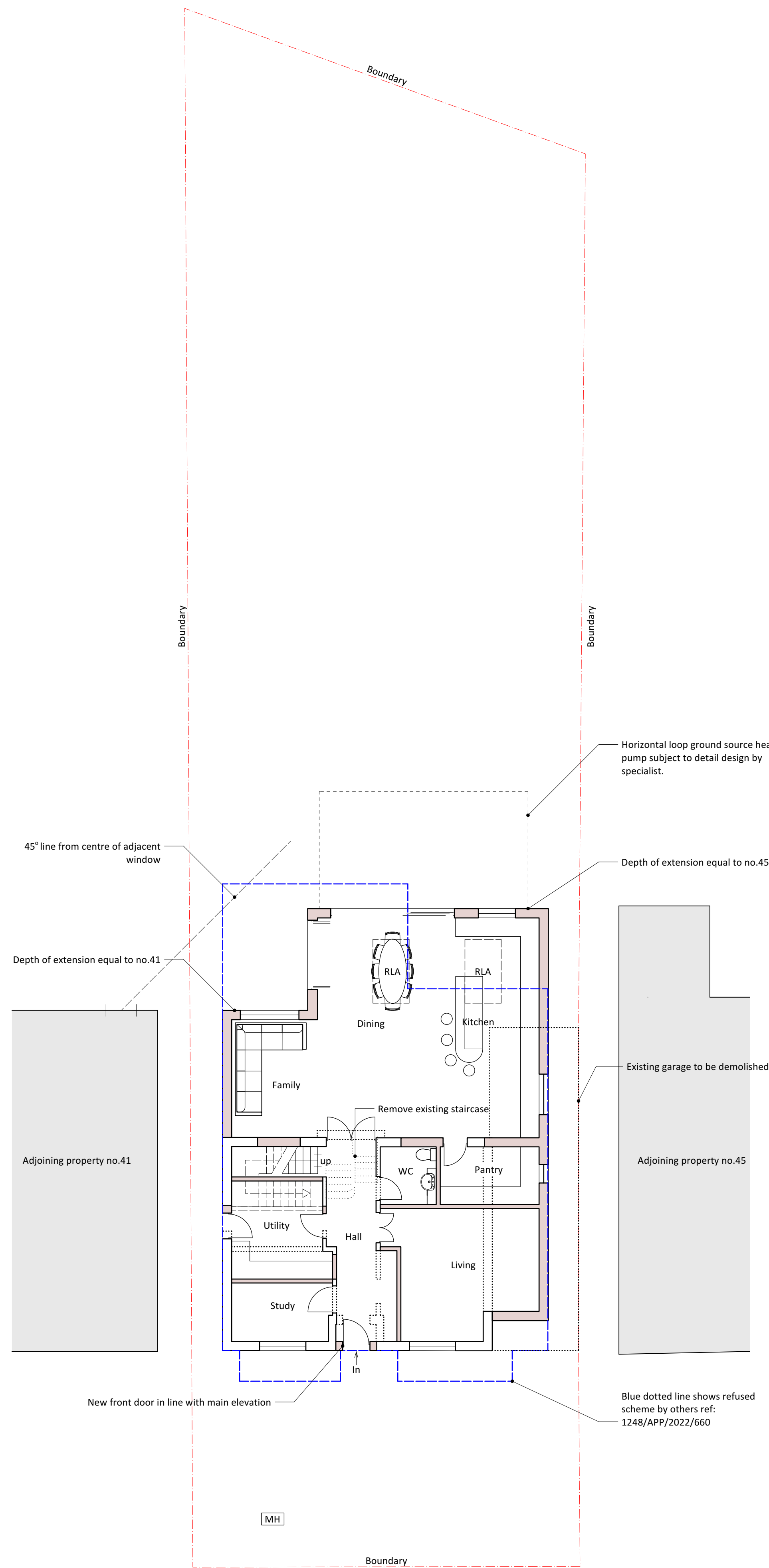
1 GROUND Scale: 1:100
