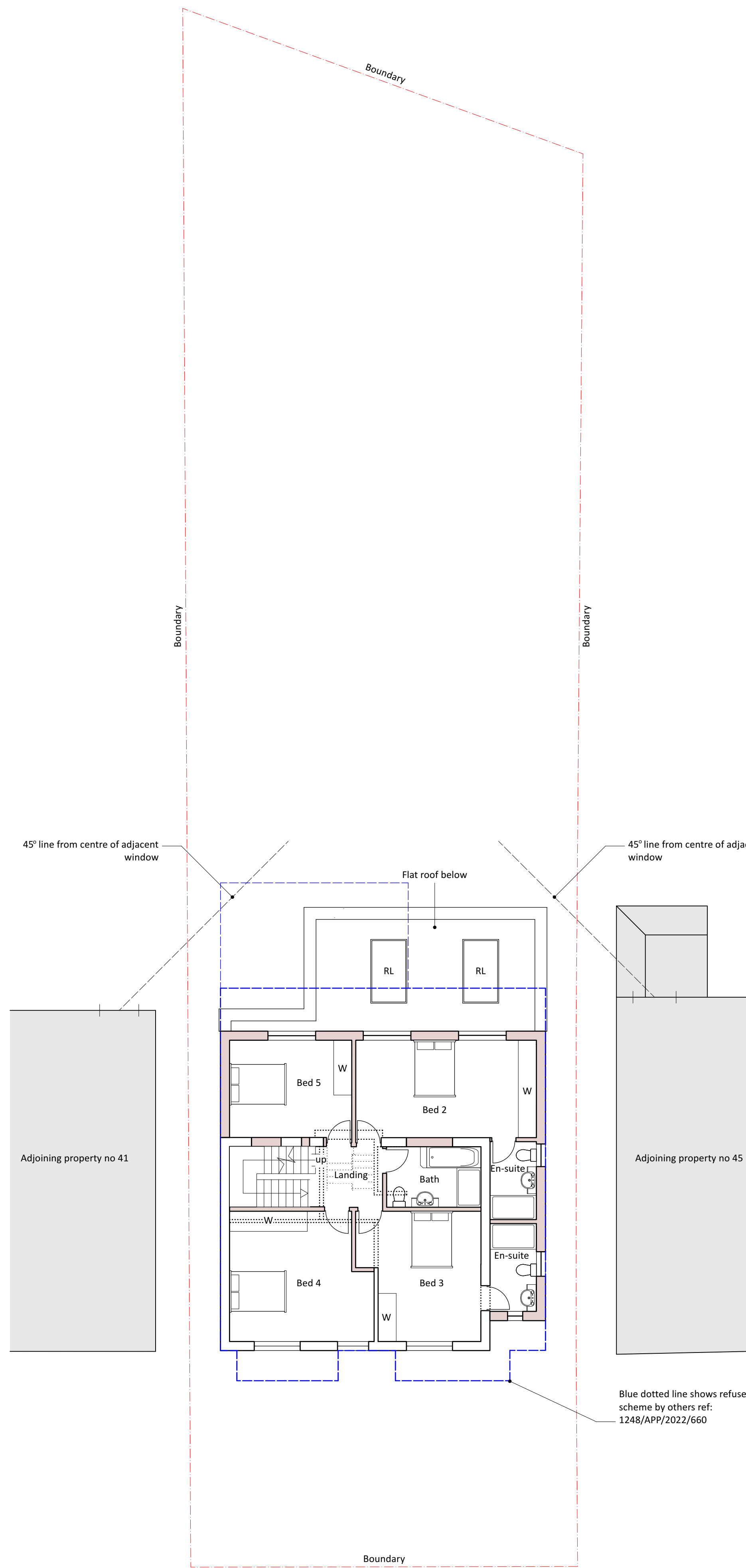
2 FIRST Scale 1:100
