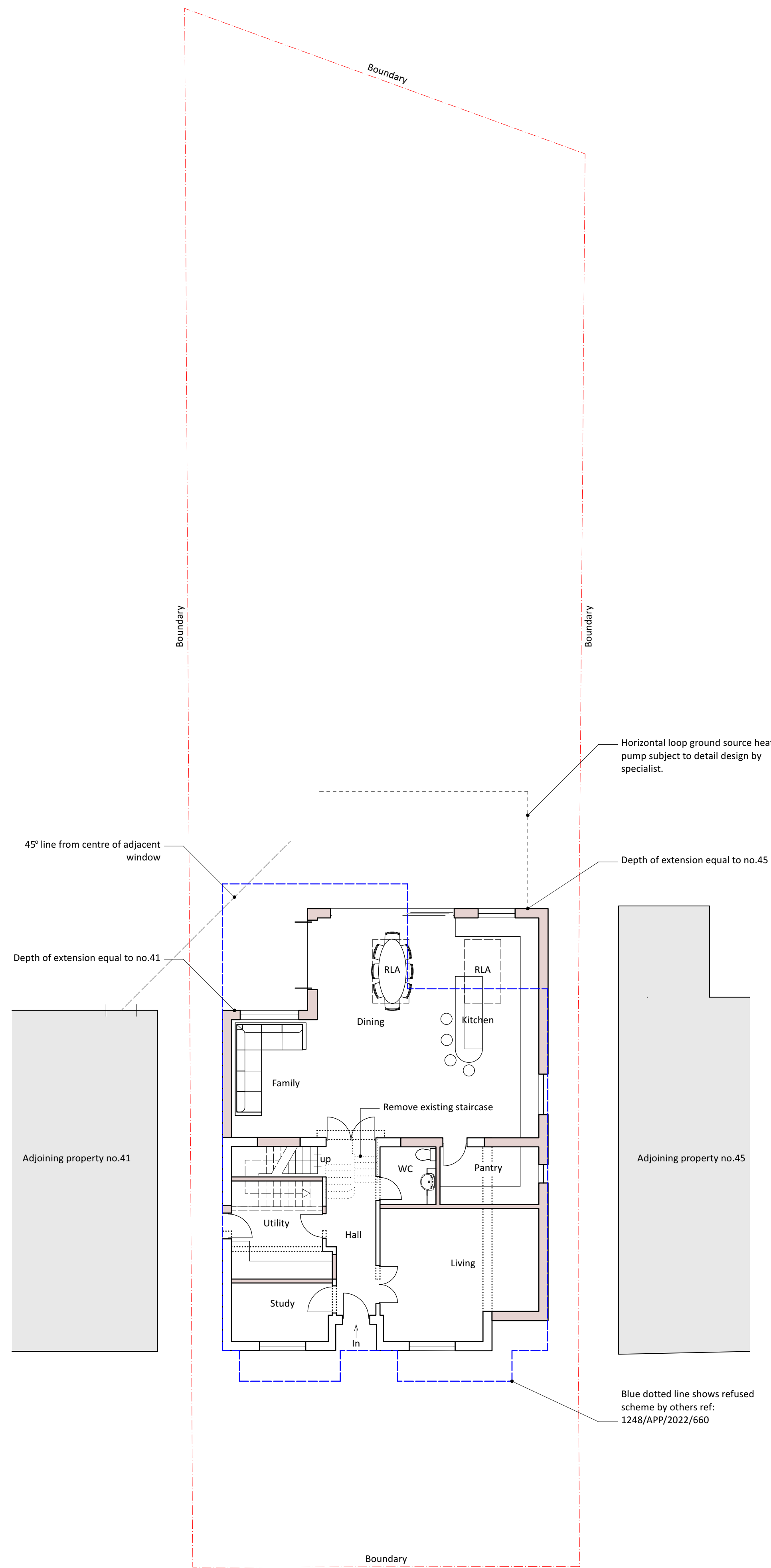
1 GROUND Scale 1:100
