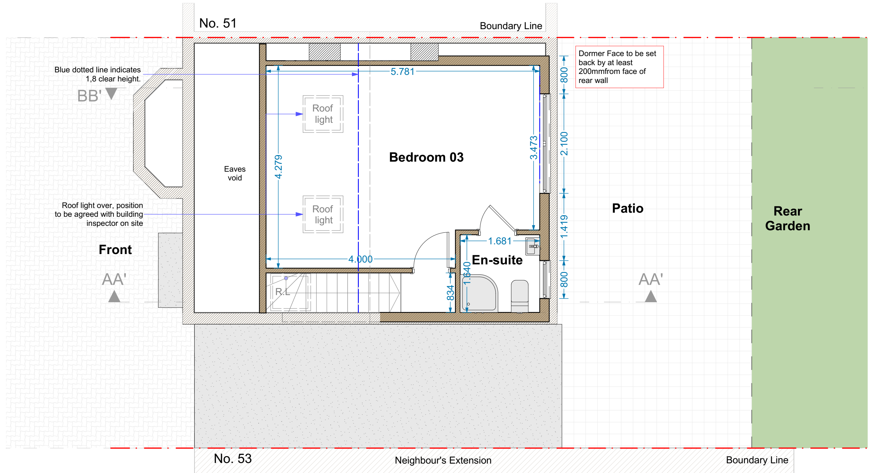
Proposed Second Floor Plan 1:50
