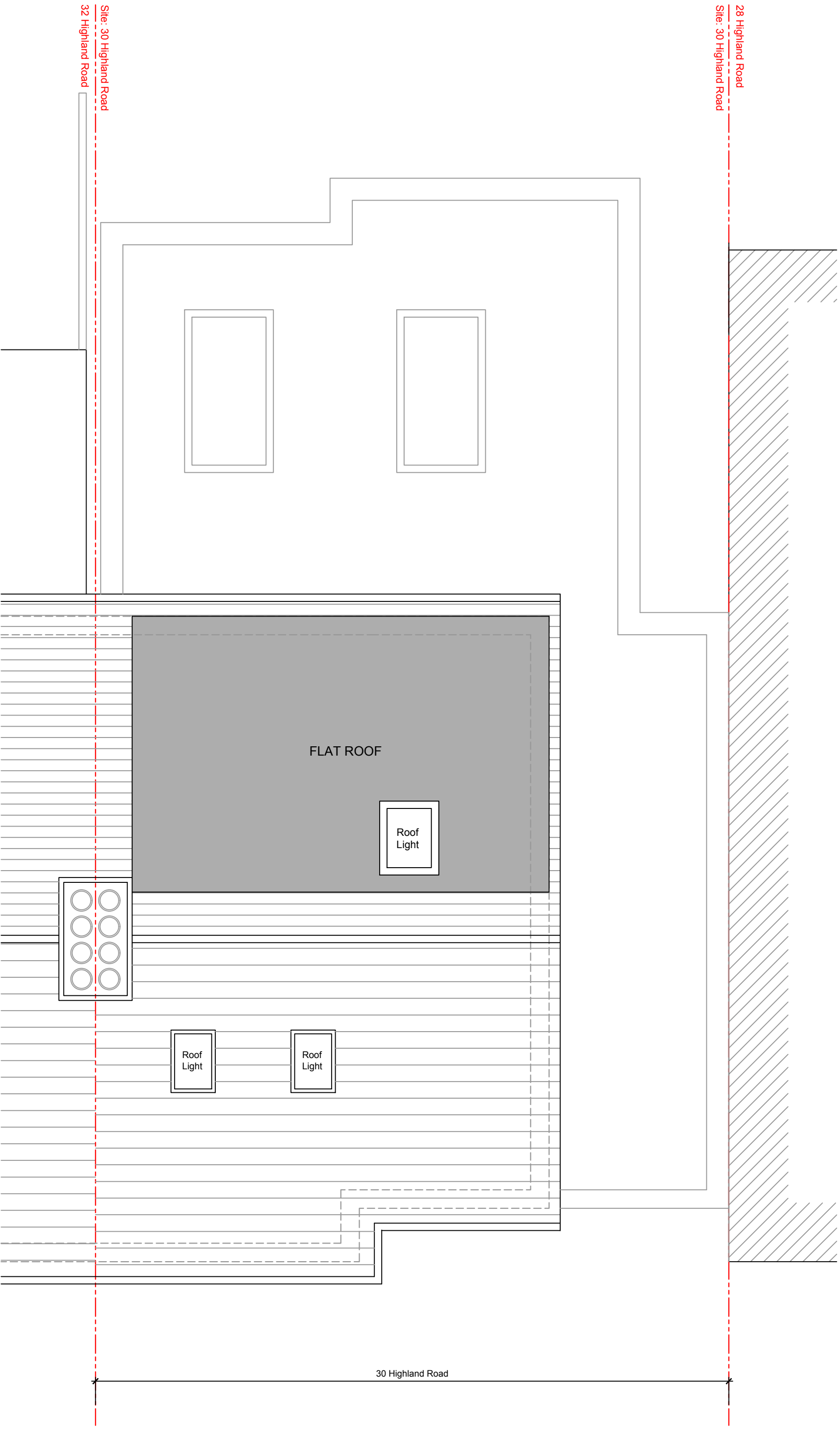
ROOF PLAN - As Proposed Scale 1:50
