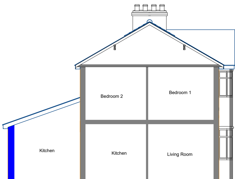
Proposed Section
