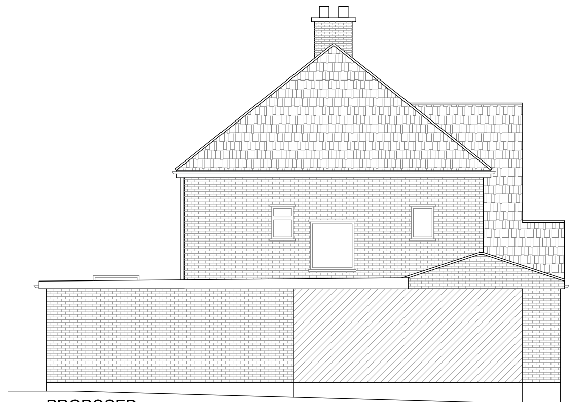
PROPOSED SIDE ELEVATION-2
