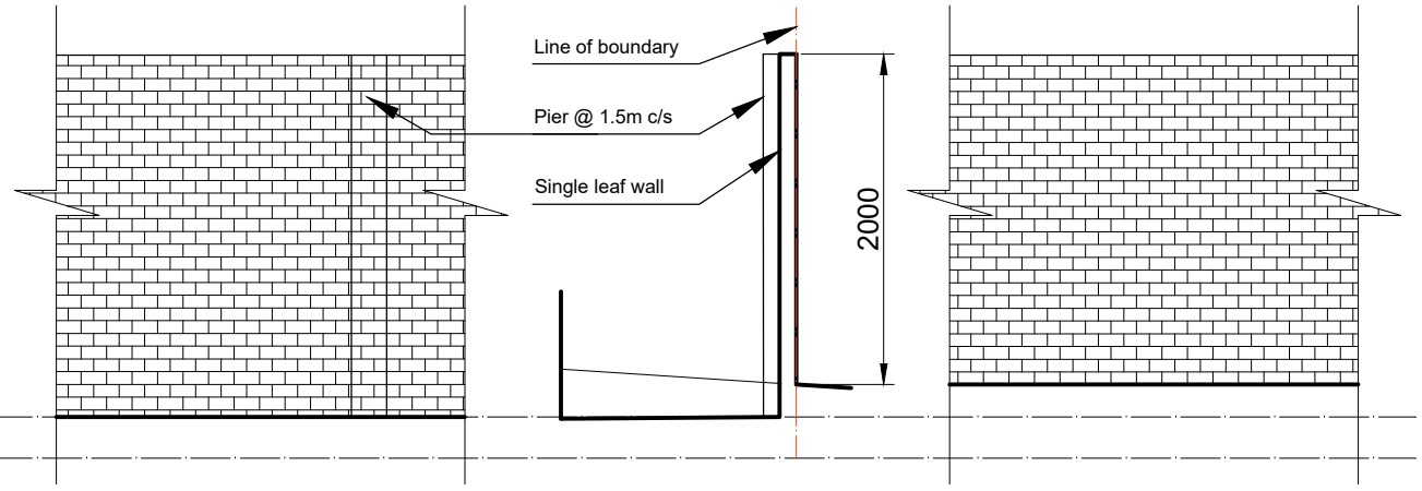
1 Boundary Wall- elevation(view from site) Scale: 1:50
