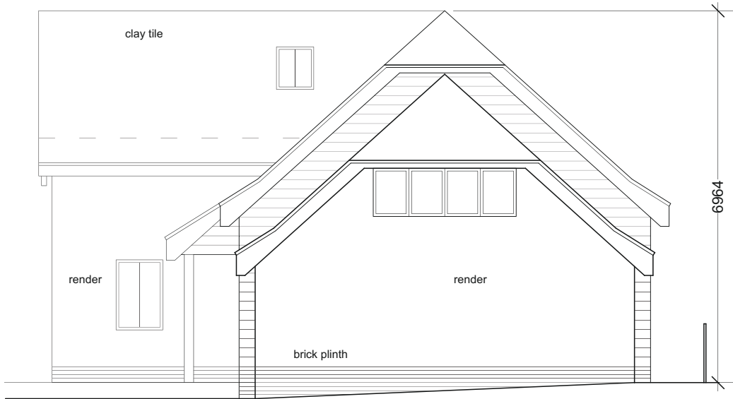
01 North Elevation 1:100@A3; 1:50@A1
