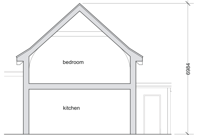
03 Section AA 1:100@A3; 1:50@A1
