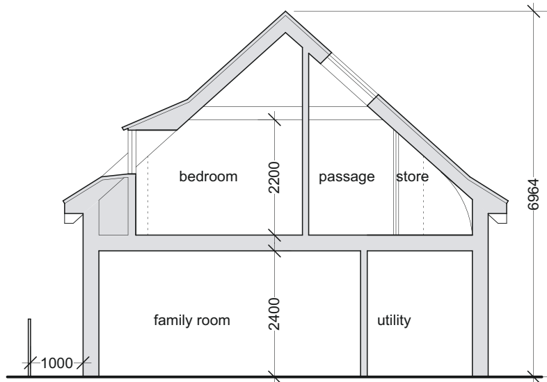
05 Section CC 1:100@A3; 1:50@A1
