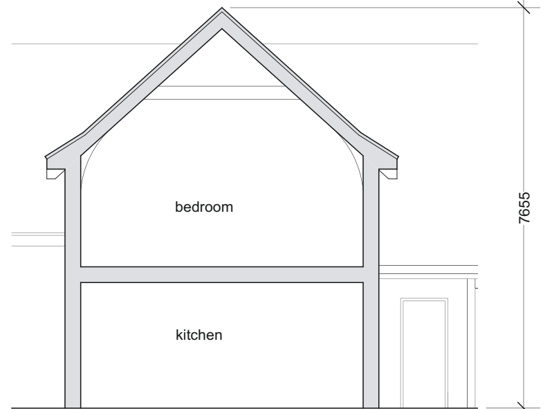
03 16 Section AA 1:100@A3; 1:50@A1
