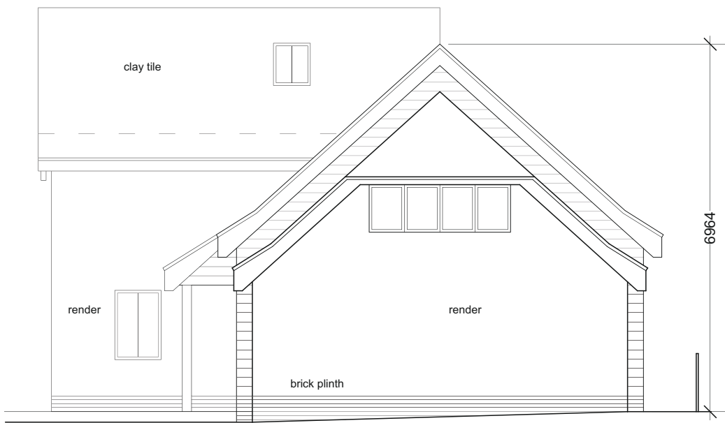
01 16 North Elevation 1:100@A3; 1:50@A1
