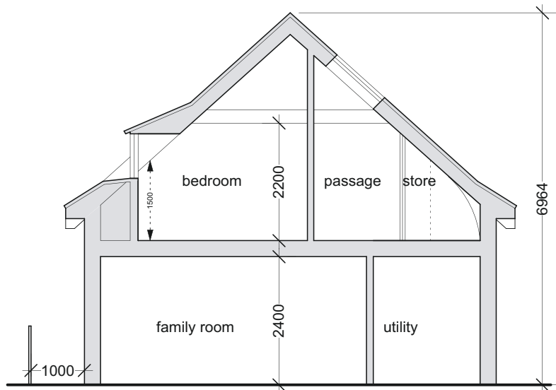
05 16 Section CC 1:100@A3; 1:50@A1
