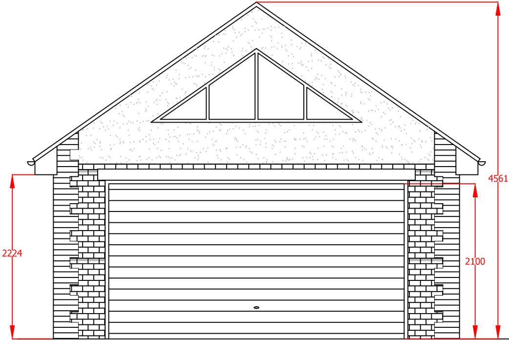
East Elevation
