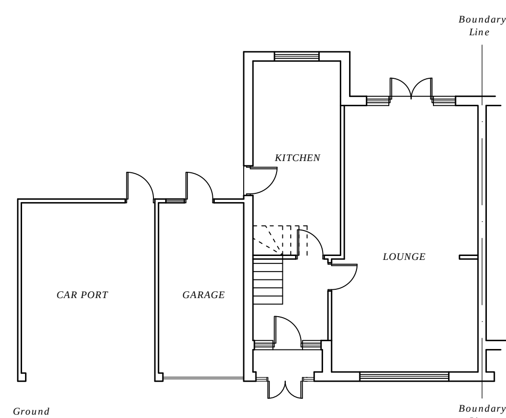
Existing Plans and Elevations
