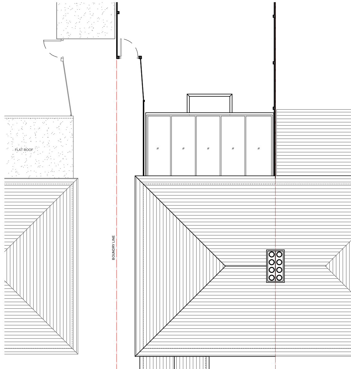
05 - ROOF PLAN
